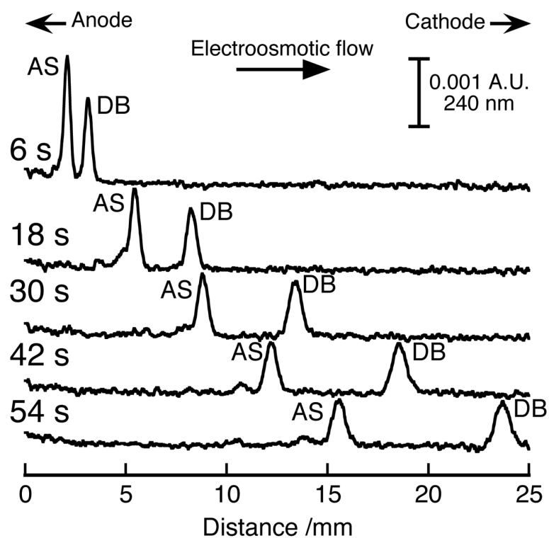
Fig. S1 Electropherograms extracted at intervals of 12 s from a series of electropherograms obtained successively in a single MCE separation run for the sample containing AS and DB.
