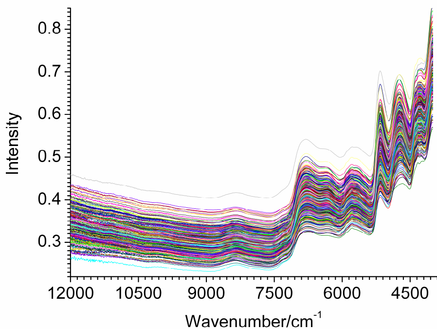
Fig. S2 Measured NIR spectra of the tobacco samples
