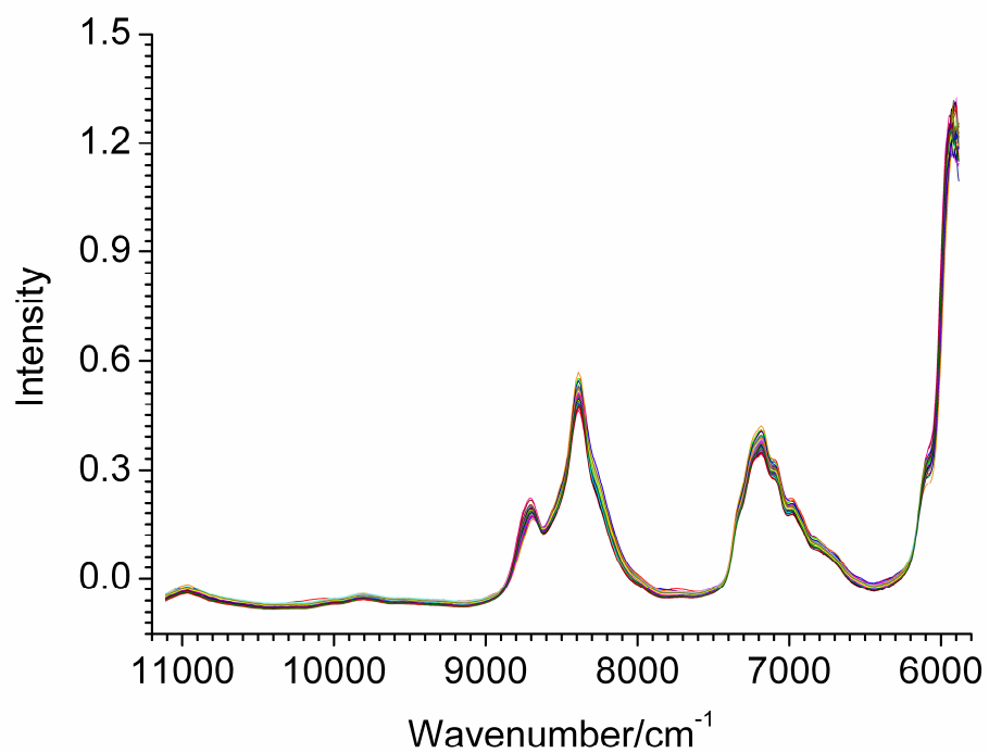
Fig. S1 Measured NIR Spectra of gasoline samples
