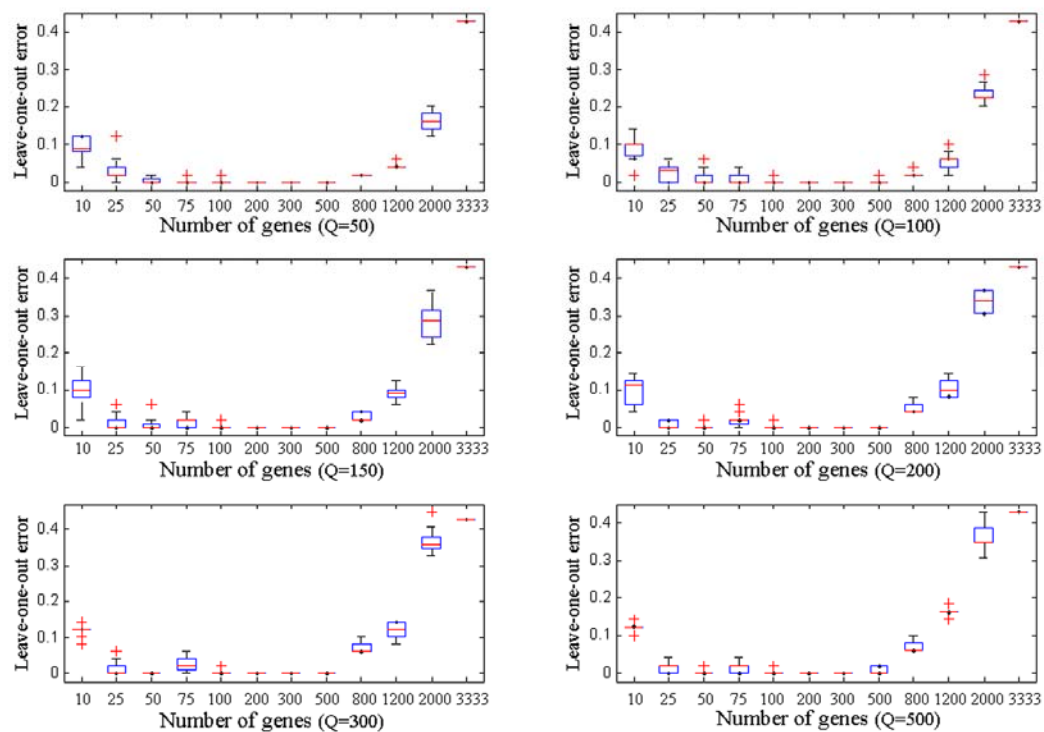
Figure S2. the results of reproducibility test of 20 runs of NISPA for estrogen dataset when Q=50, 100, 150, 200, 300 and 500 , respectively.
