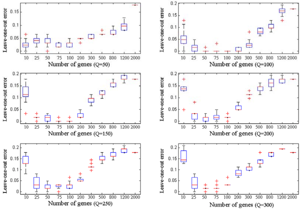
Figure S1. the results of reproducibility test of 20 runs of NISPA for colon dataset when Q=50, 100, 150, 200, 250 and 300 , respectively.
