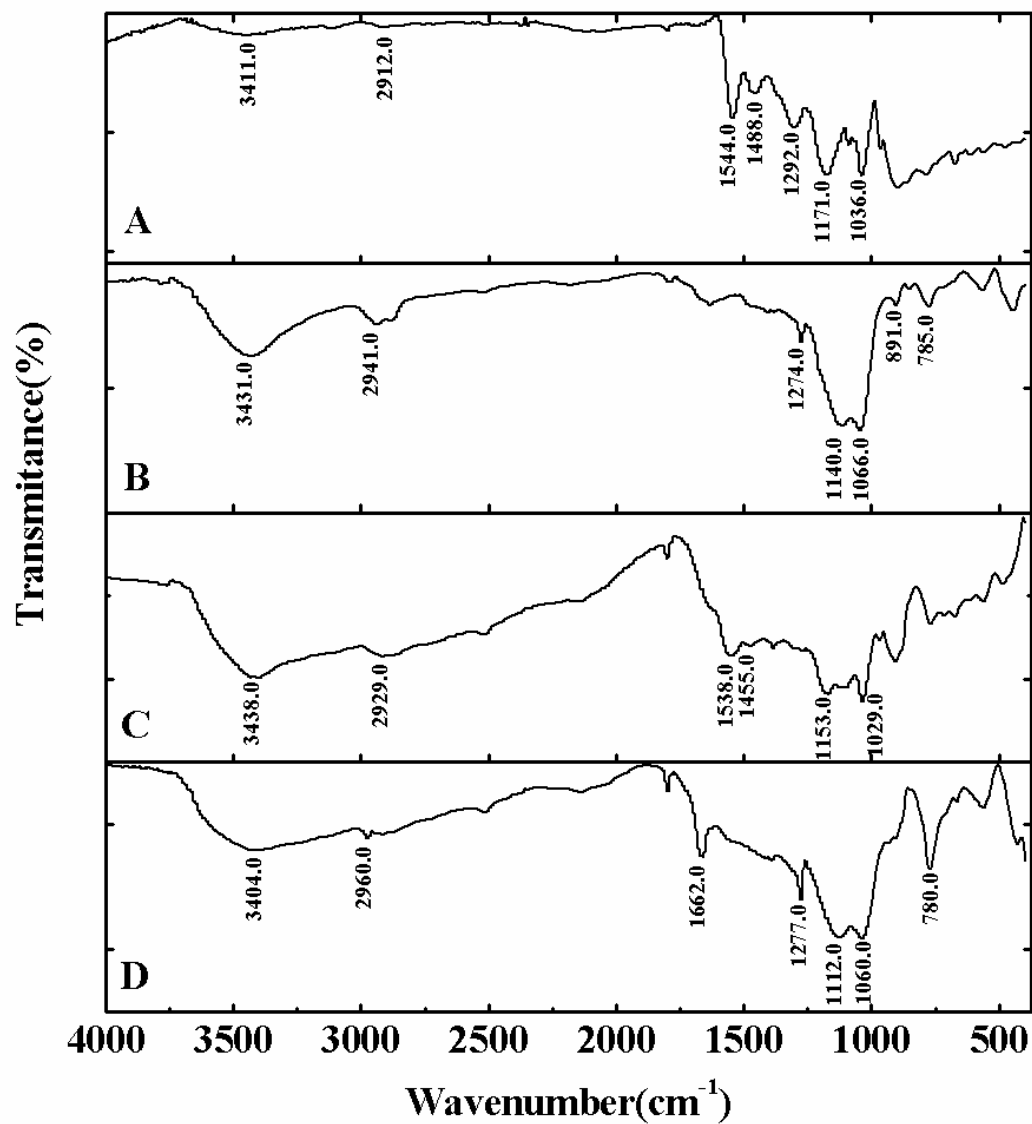
Fig. 1s Fourier IR absorption spectra of PPy/ \beta -NSA (A: before sol-gel reaction, B: after sol-gel reaction) and PPy/GR (C: before sol-gel reaction, D: after sol-gel reaction) SPME fiber coating
