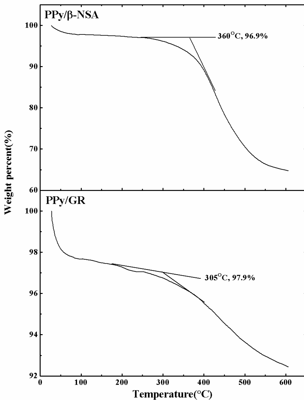
10 Fig. 2s Thermogravimetric analysis curves for PPy/β-NSA and PPy/GR SPME fiber
