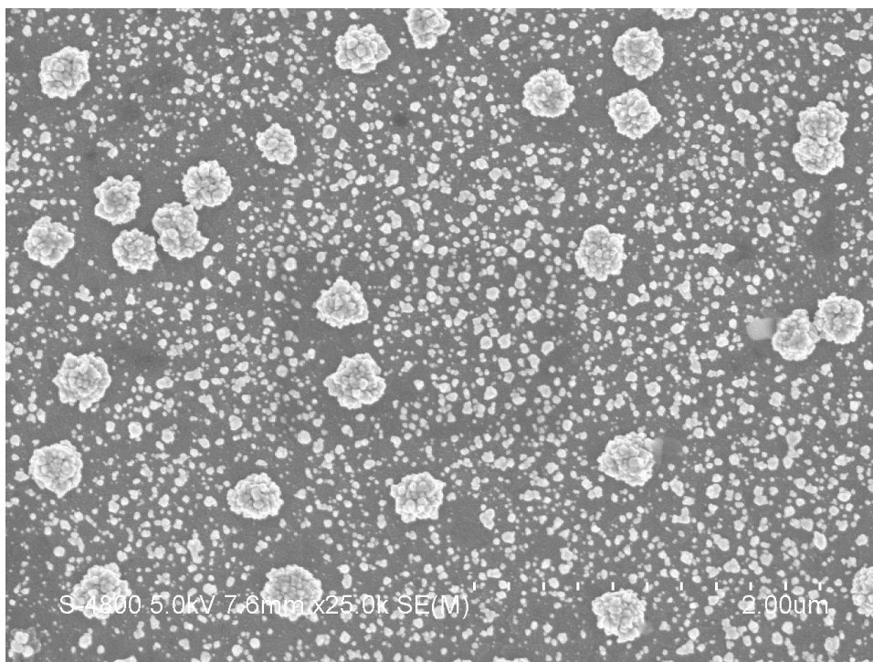
Figure S1 FE-SEM image of Au nanoflowers modified on the Cys/Au electrode surface.
