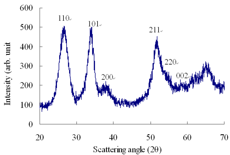
XRD patterns of the SnO 2 nanoparticles
