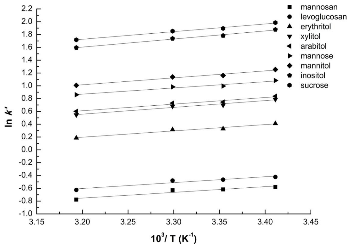
Van't Hoff plots in the temperature range of 20-40°C. Mobile phase: ACN/water 90/10 (v/v) in formic acid 10mM. Chromatographic column: HILIC-diol.
