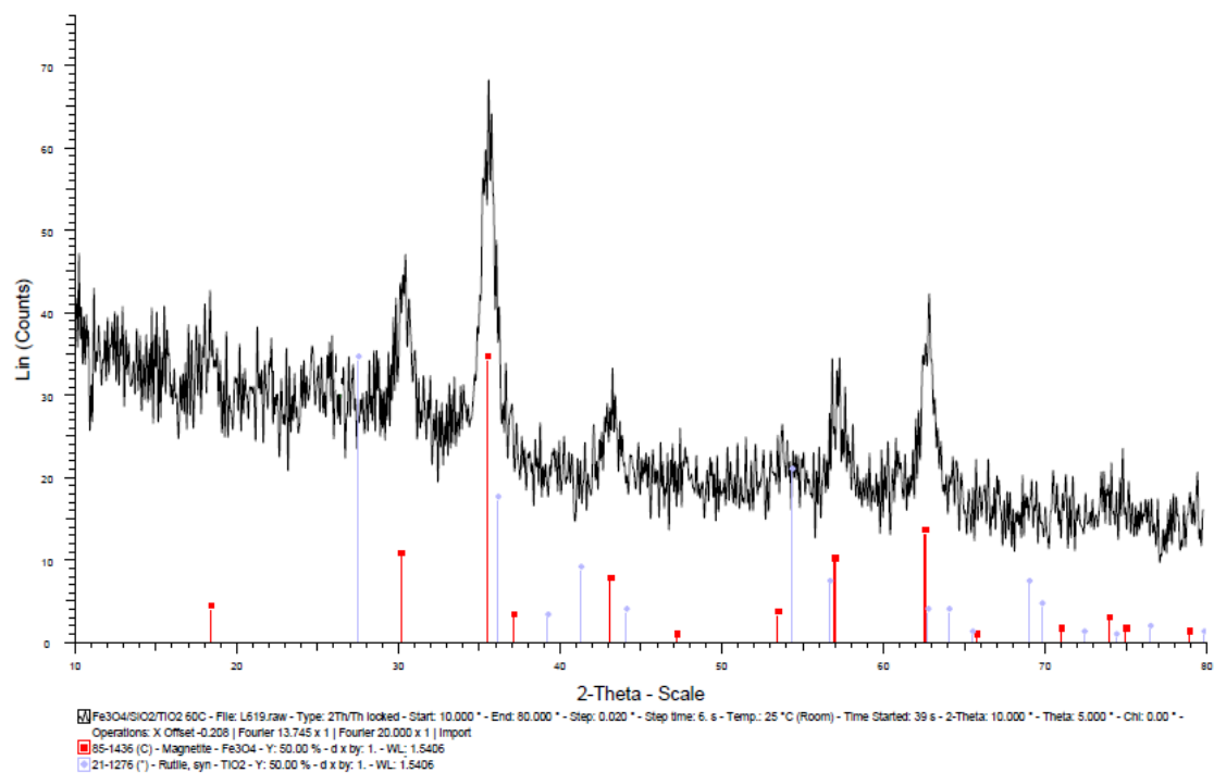
XRD of iron oxide/silica/titania material
