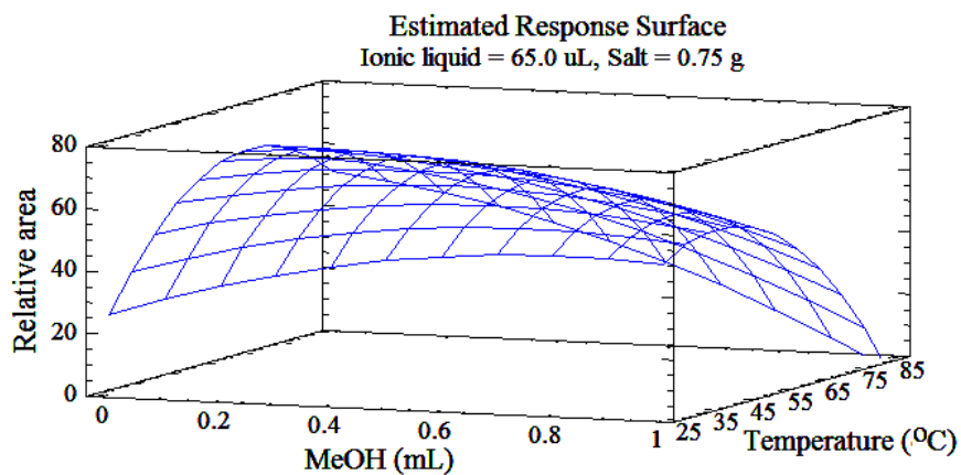
Fig. 1s: Response surface estimated from the Box-Behnken design for significant interaction effects such as: volume of MeOH vs extraction temperature
