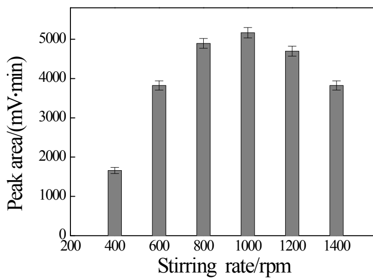
Fig. S1 Effect of stirring rate on the extraction efficiency of BPA.
