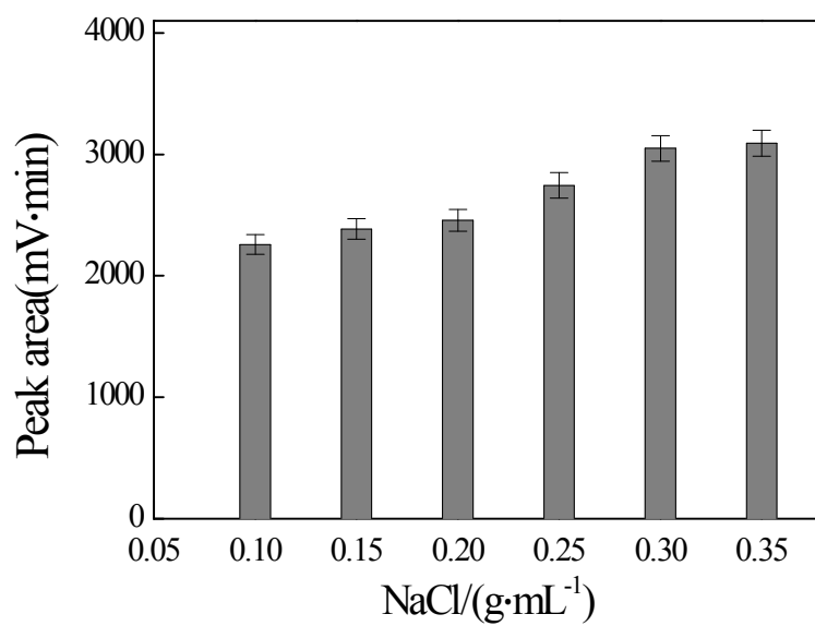
Fig. S2 Effect of NaCl concentration on the extraction efficiency of BPA.
