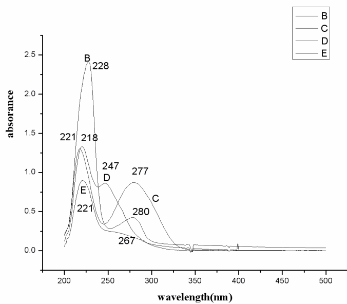
Fig. 3. Absorption spectra of BSA (curve B), PCB12-BSA (curve C), PCB37-BSA (curve D), PCB77-BSA (curve E) conjugates 0.01 mol L -1 in 0.02 mol L -1 PH 7.4 PBS solutions
