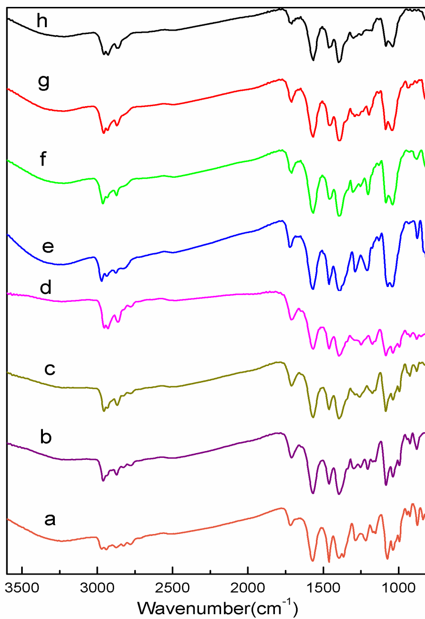
Fig. S1 Infrared spectroscopy of ILs: a. [DMEA][Pr], b. [DMEA][Bu], c. [DMEA][Pent], d. [DMEA][Hex], e. [DEEA][Pr], f. [DEEA][Bu], g. [DEEA][Pent], h. [DEEA][Hex].
