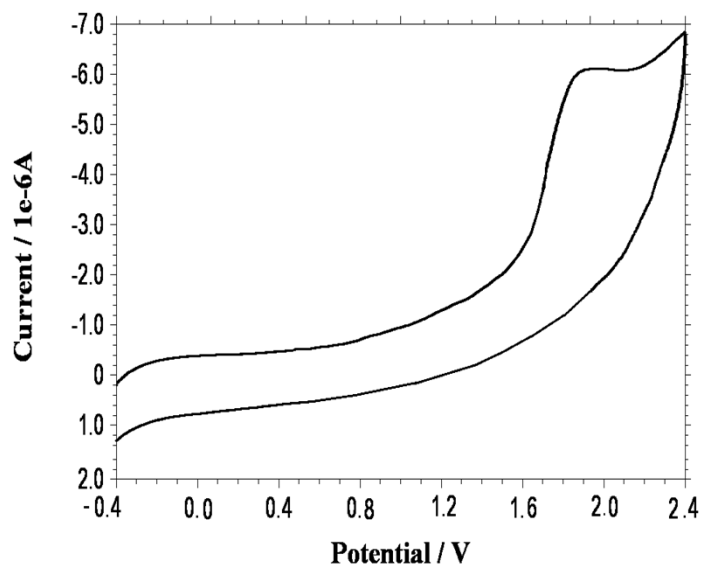
CV and DPV of CAF
