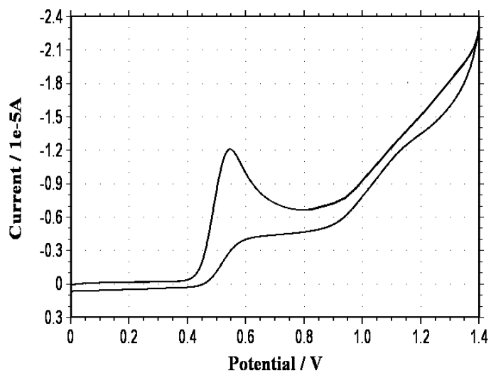
CV and DPV of CAF
