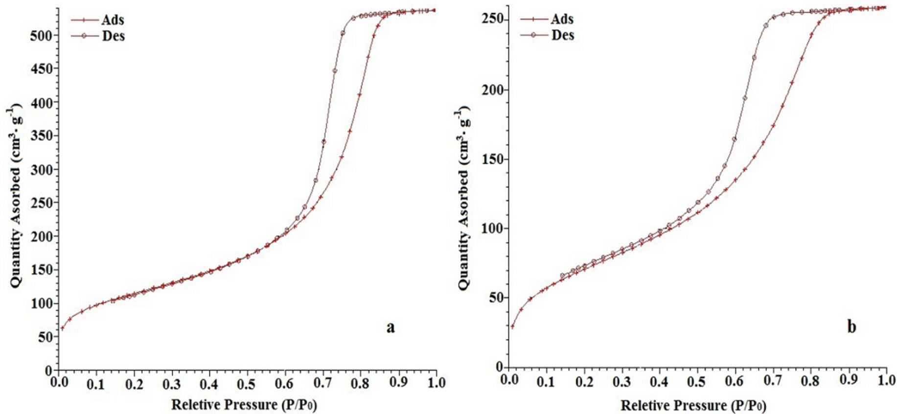
Figure 1 N_2 adsorption and desorption isotherms of activated silica gels (a) and SMIPs (b)
