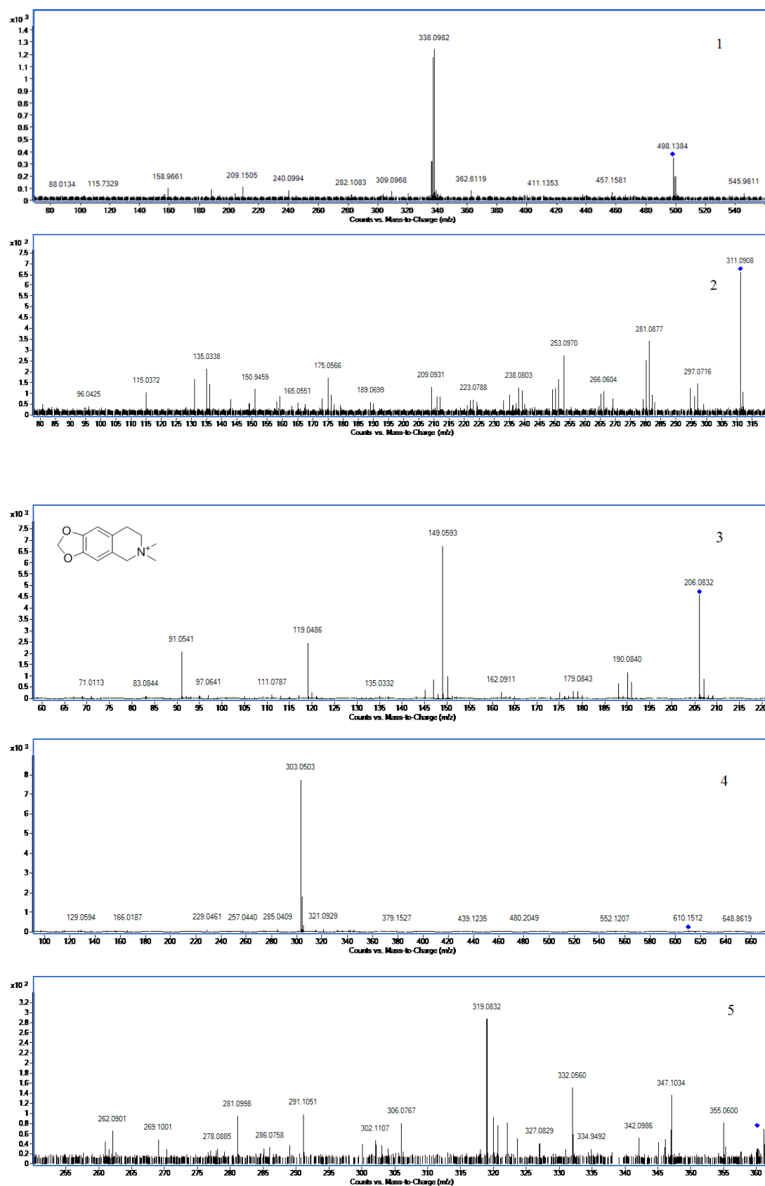
Fig. S1 ESI-MS/MS spectrum of 12 biomarker compounds.
