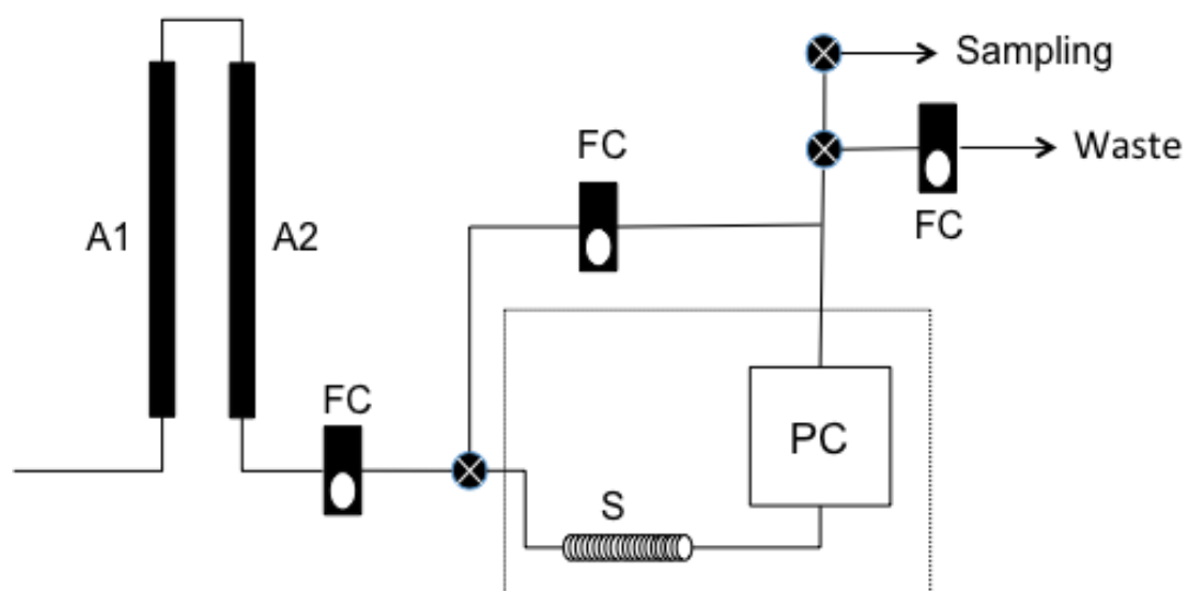
Figure S1. Standard gas generation system.
