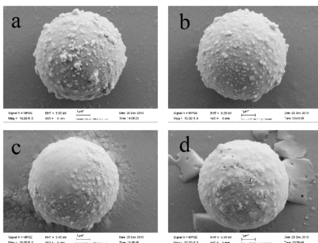
Fig. S1. Micrographs of the MBs in different reaction stages (SEM, 10,000 \times ).
