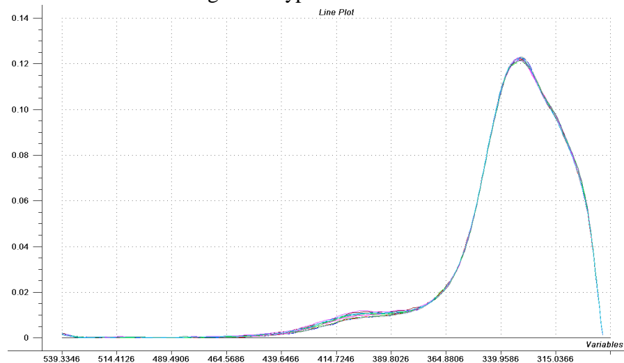
Line plot of the spectral acquisitions made in the central part of one single cell type I of the soleus muscle
