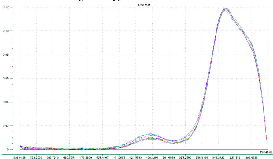
Line plot of the spectral acquisitions made in the central part of one single cell type IIX-IIB of the EDL muscle
