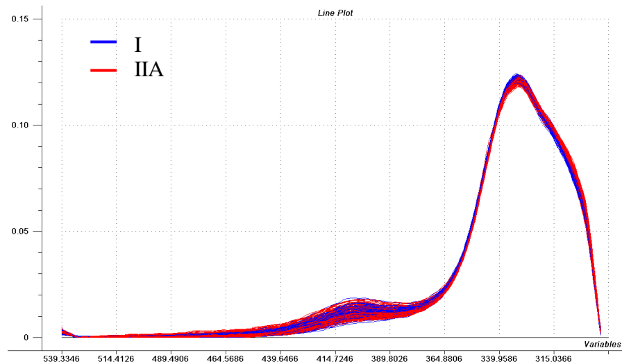
Line plot of the spectral acquisitions made in the central part of the soleus muscle
