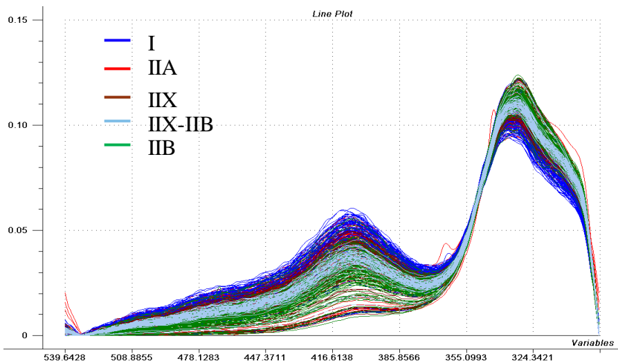
Line plot of all the spectral acquisitions made in the central part of the EDL muscle
