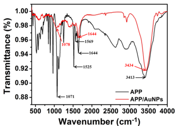
Figure S1. FT-IR spectra of APP and APP/AuNPs.
