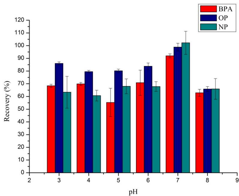
Figure S3 Effect of solution pH on the recoveries of three PEEs (n =6)
