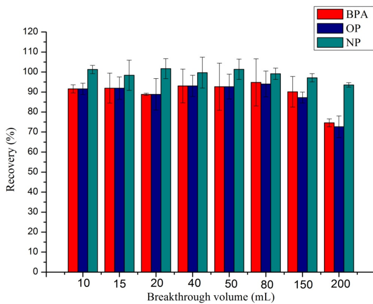
Figure S4 Effect of sample volume on the recoveries of three PEEs (n =6)
