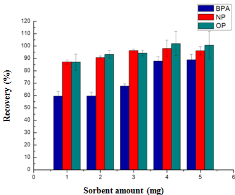
Figure S2 Effect of amount of HM-PAN nanofibers mat on the recoveries of three PEEs (n =6)
