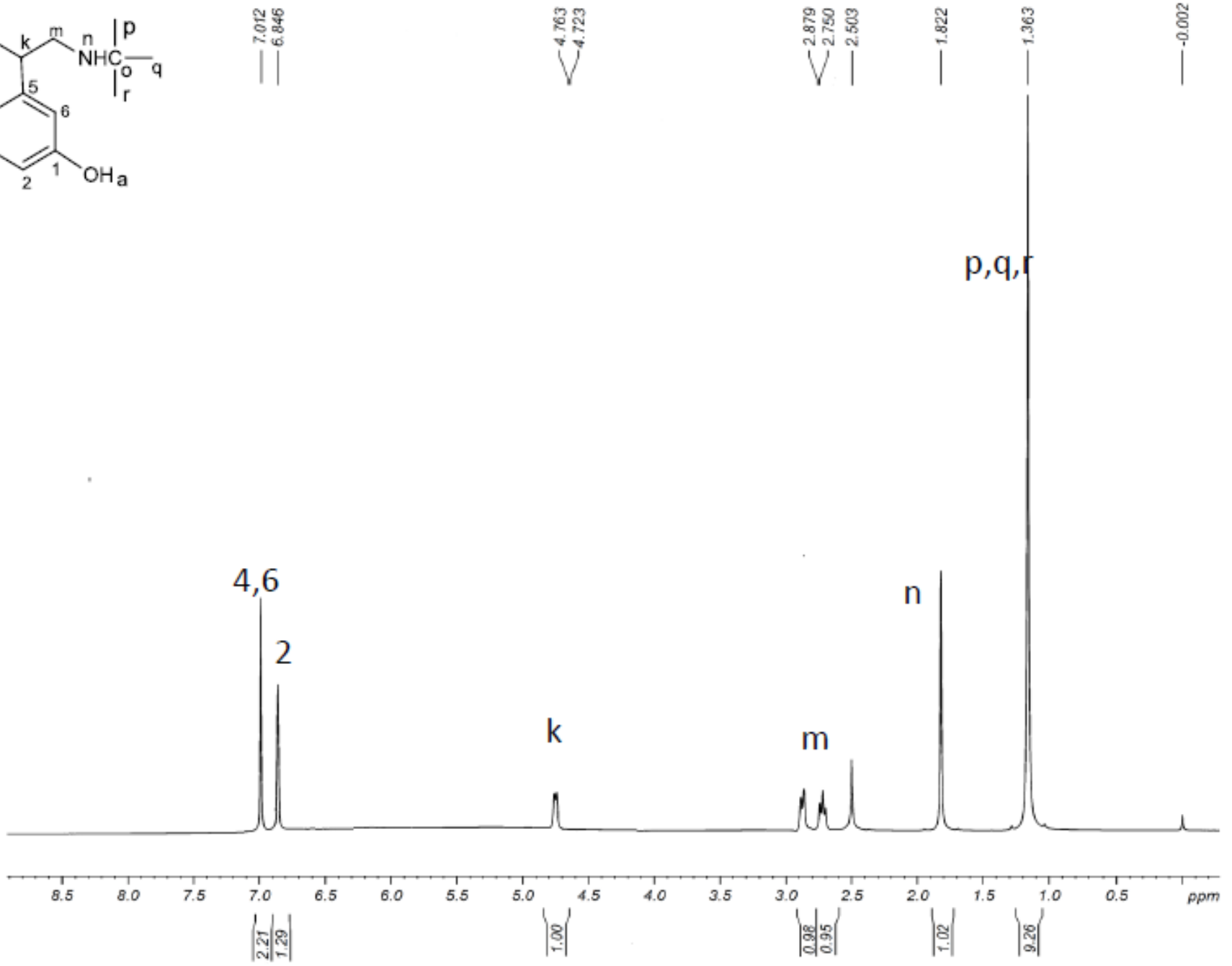
Sfigure 8: 1 H NMR spectra of DP-3
