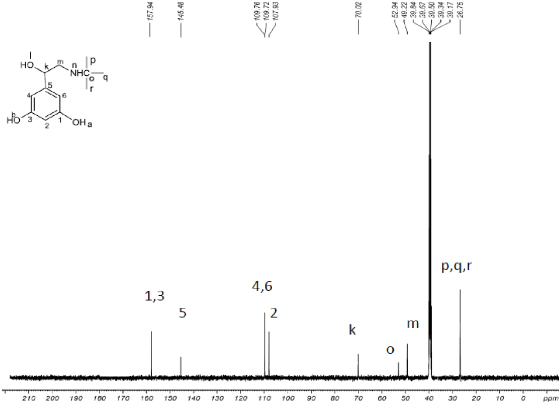
Figure 9: ^{13}\text{C} NMR spectra of DP-3
