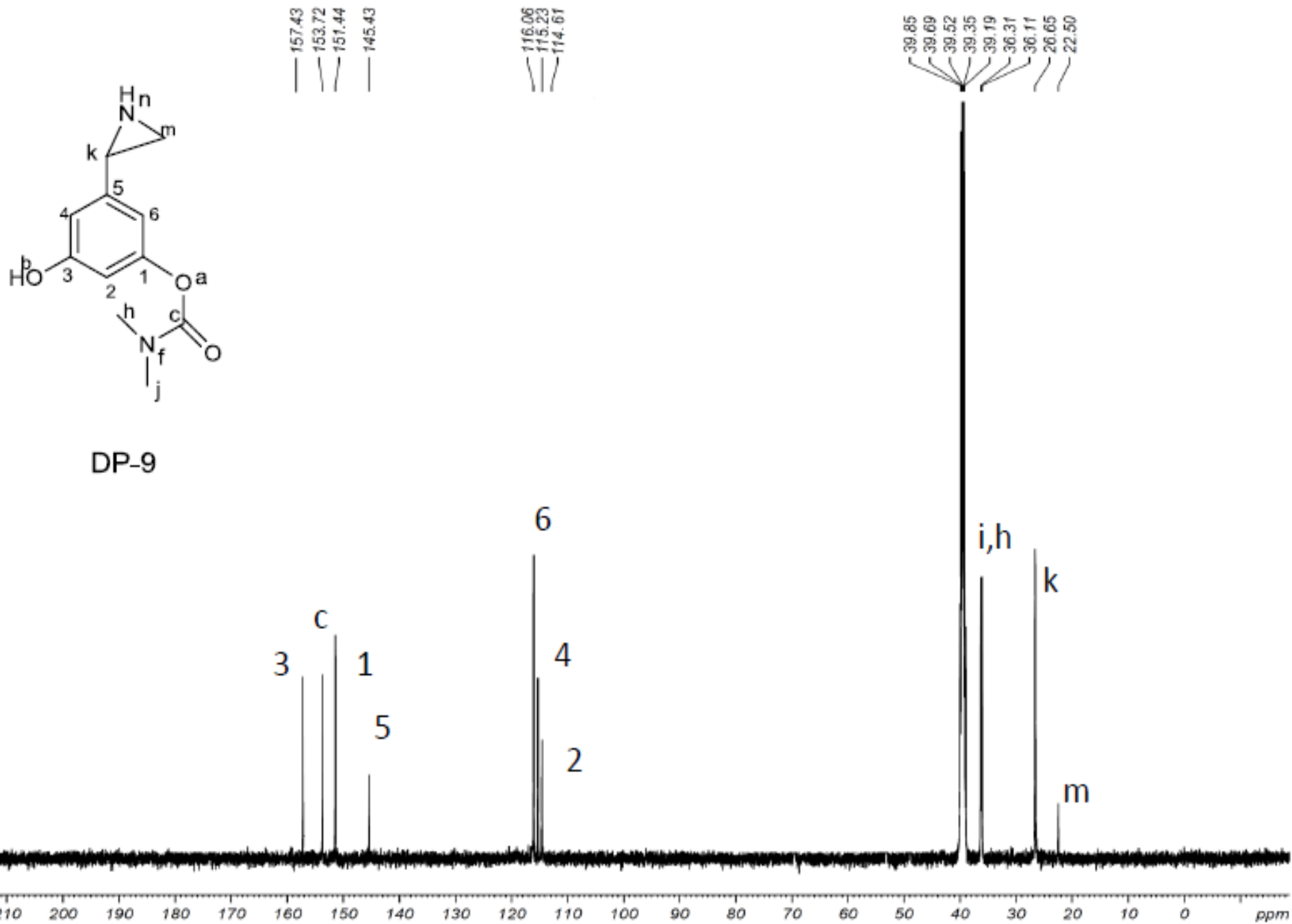
Figure 24: 13 C NMR spectra of DP-9
