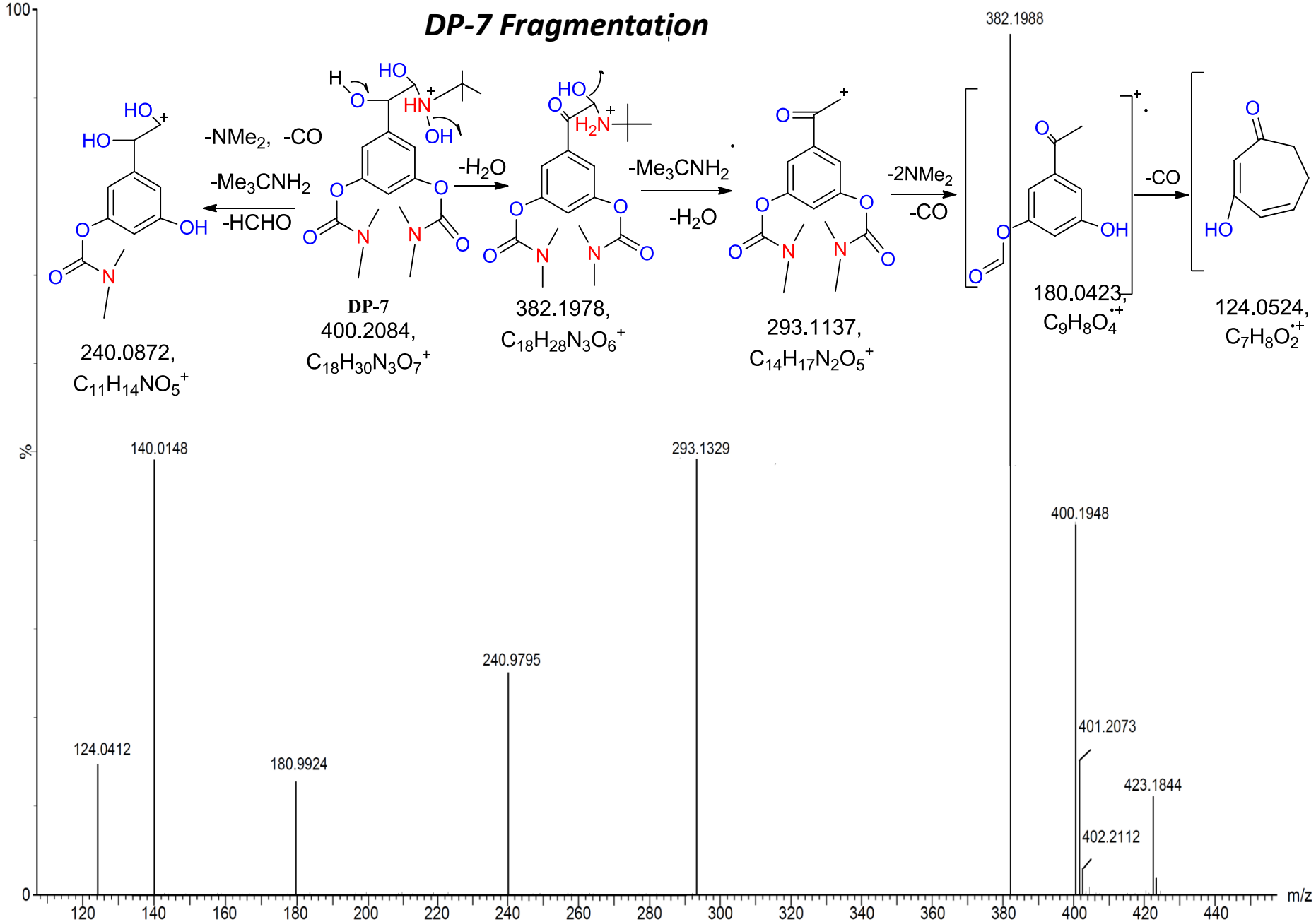
Figure 21: Fragmentation pattern and LCMS spectra of DP-7
