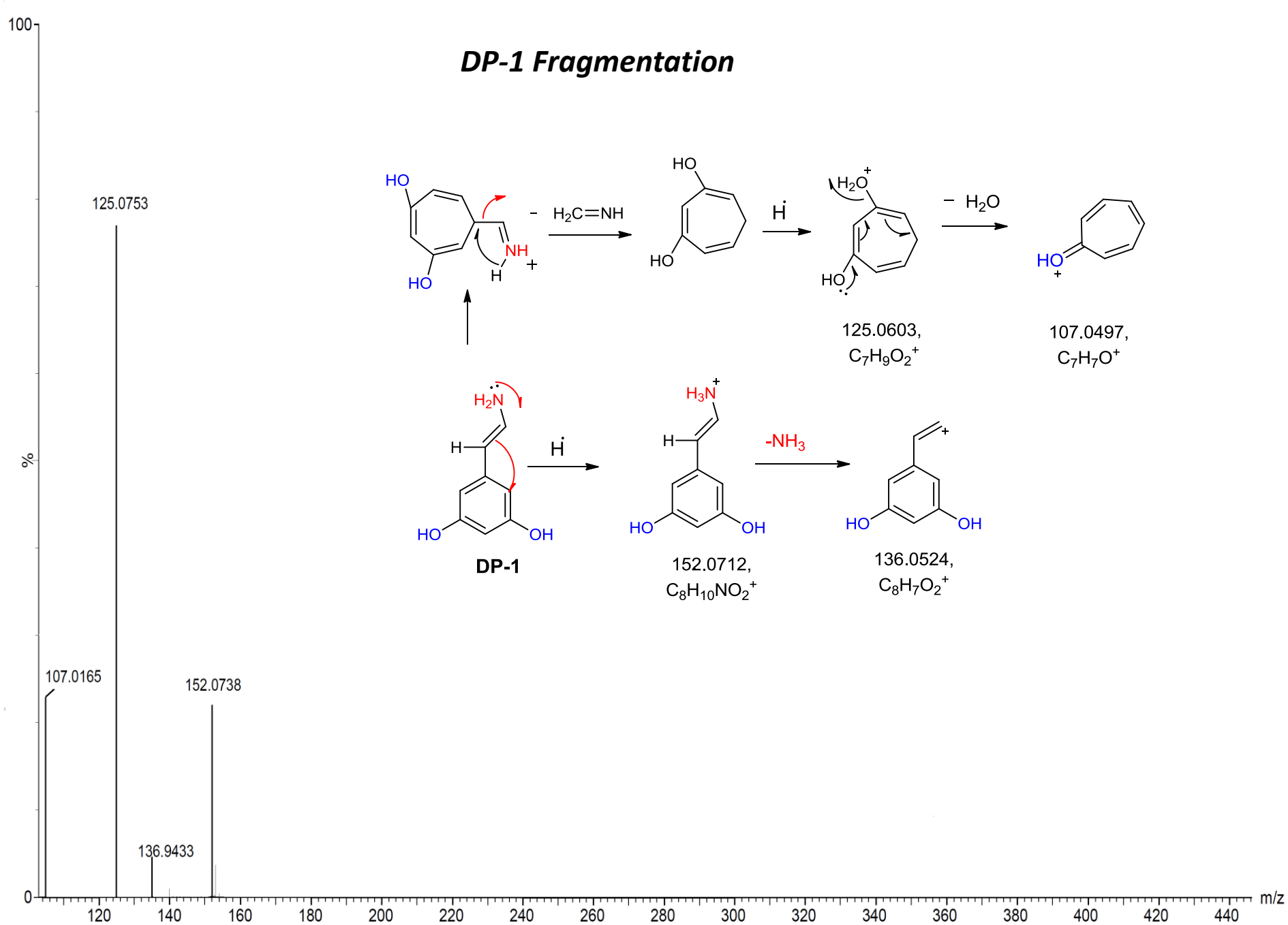
Figure 6: Fragmentation pattern and LCMS spectra of DP-1
