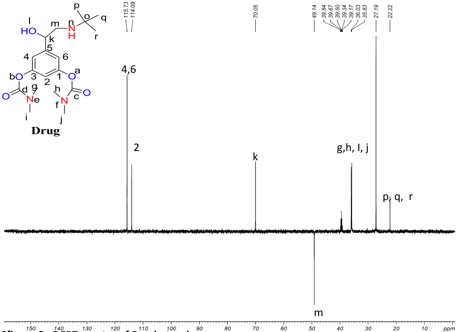
Figure 2: DEPT spectra of Bambuterol
