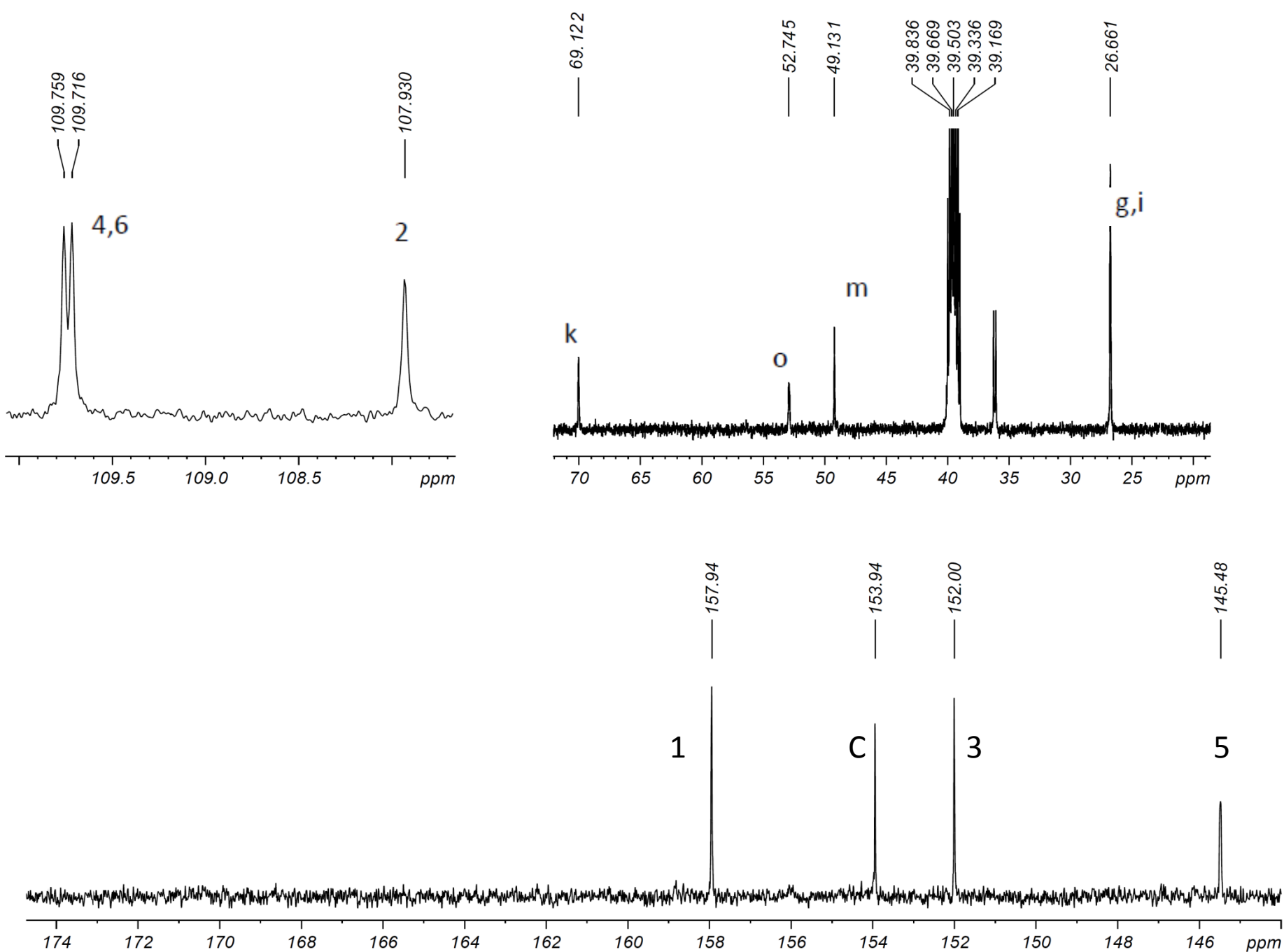
Figure 15: ^{13}\text{C} NMR expanded spectra of DP-4
