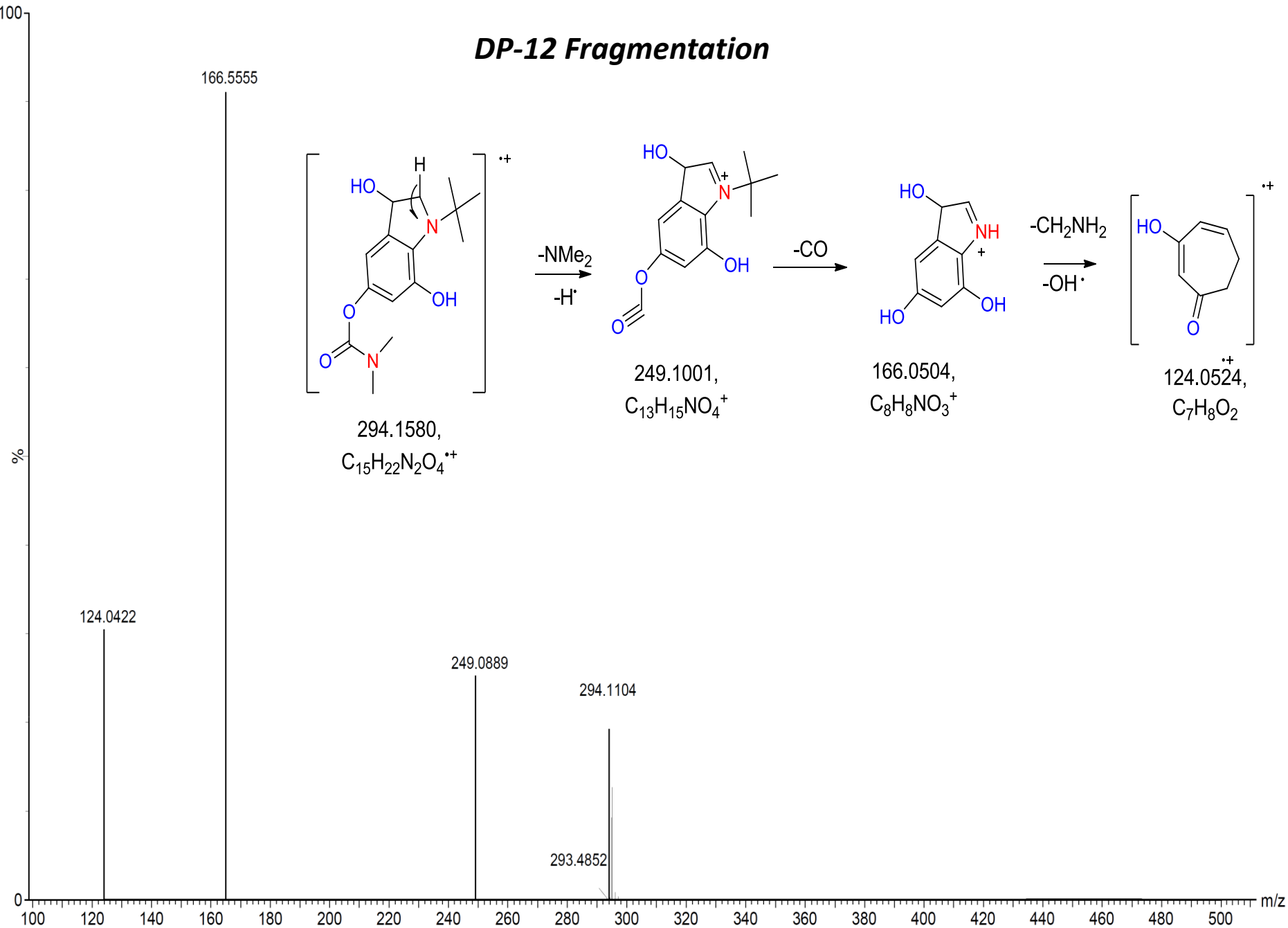
Figure 29: Fragmentation pattern and LCMS spectra of DP-12
