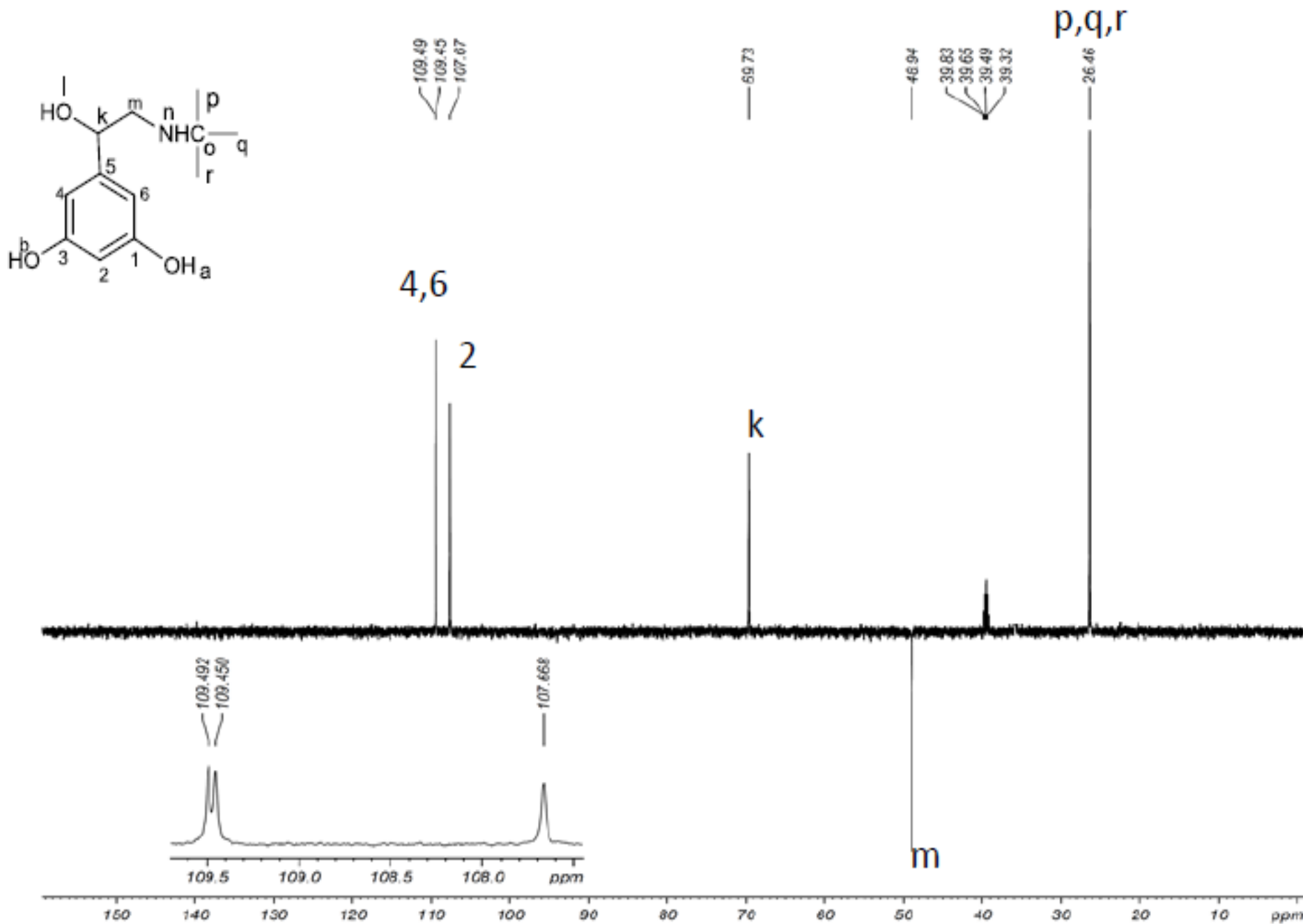
Figure 10: DEPT-135 NMR spectra of DP-3
