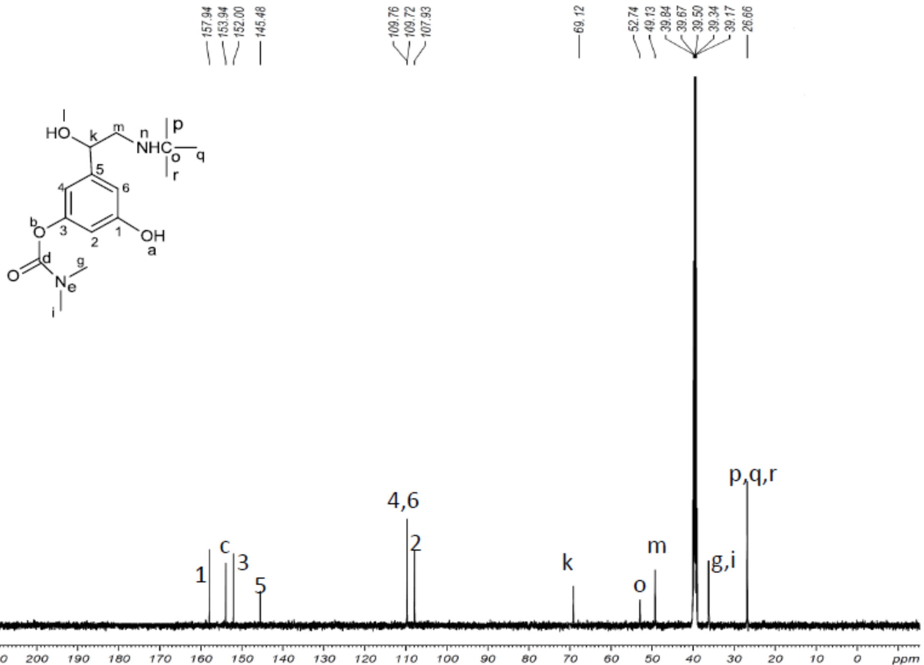
Figure 14: ^{13}\text{C} NMR spectra of DP-4
