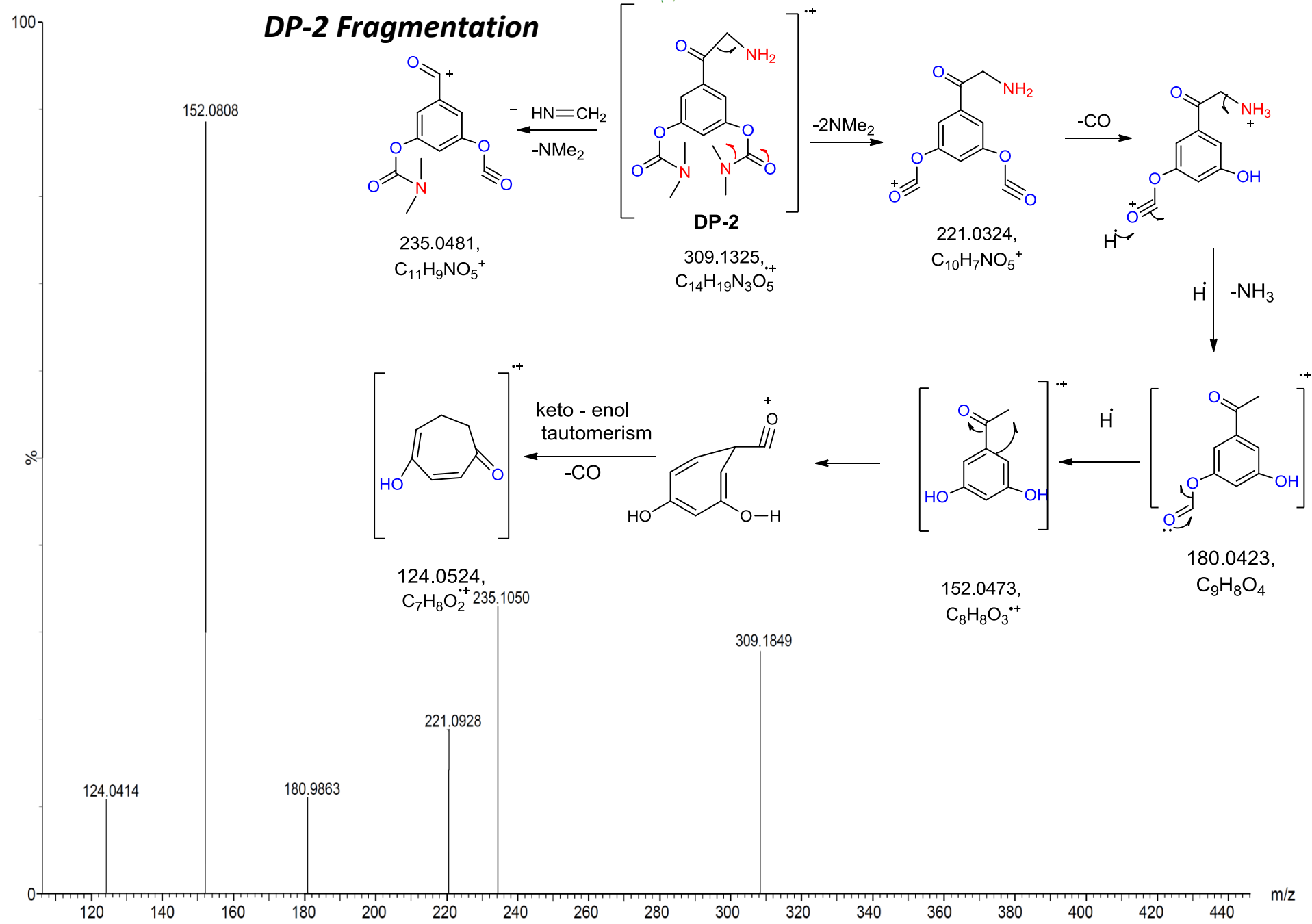
Figure 7: Fragmentation pattern and LCMS spectra of DP-2
