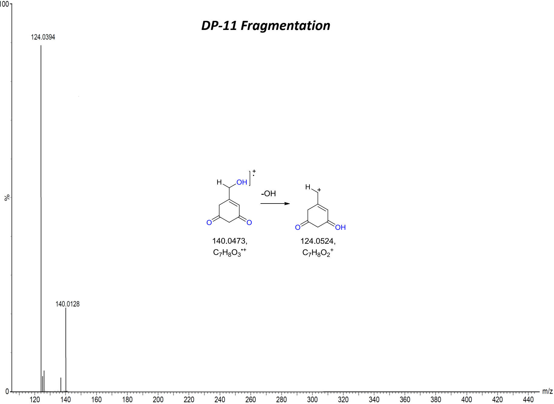
Sfigure28 : Fragmentation pattern and LCMS spectra of DP-11
