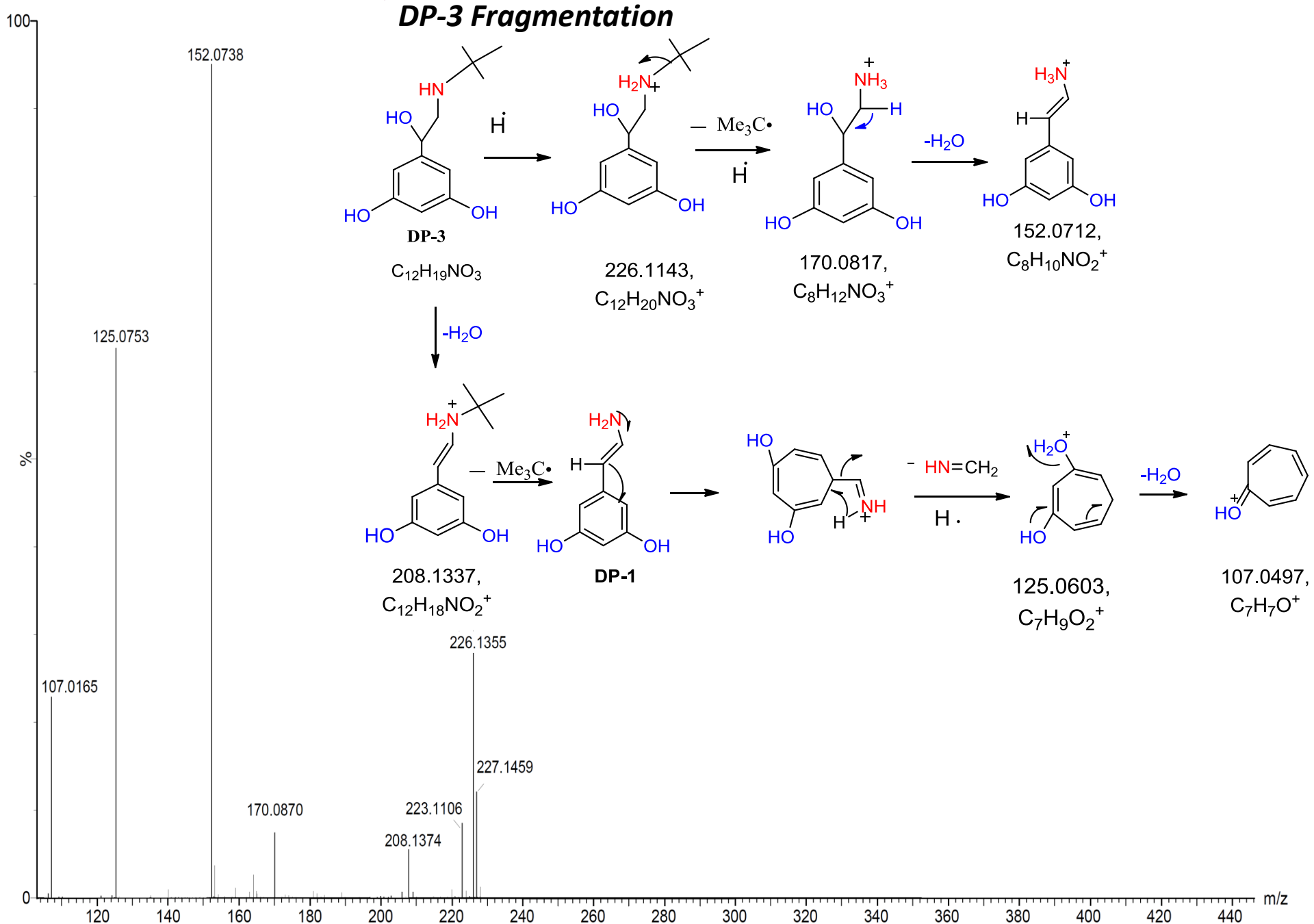
Figure 12: Fragmentation pattern and LCMS spectra of DP-3
