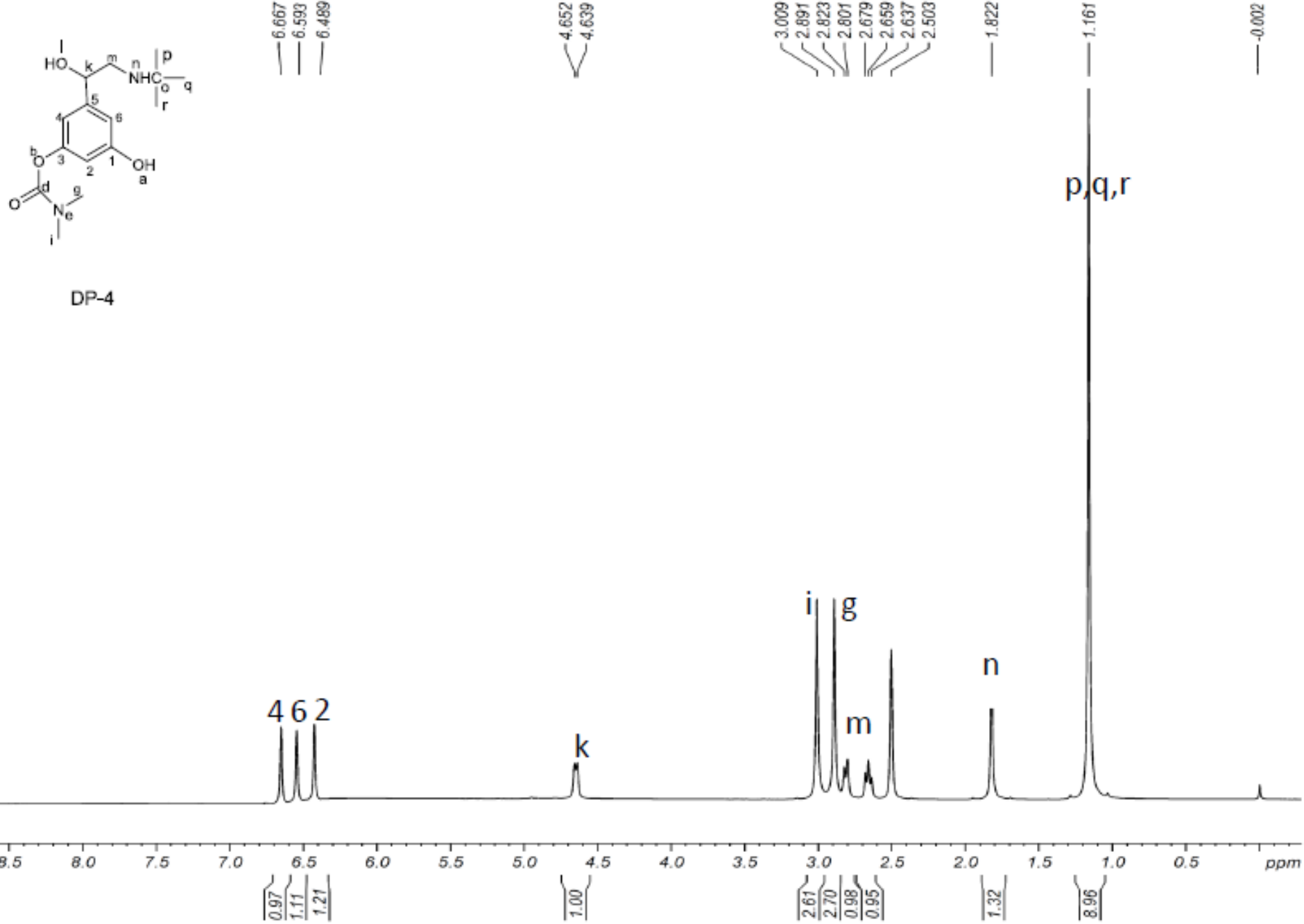
Sfigure 13: 1 H NMR spectra of DP-4
