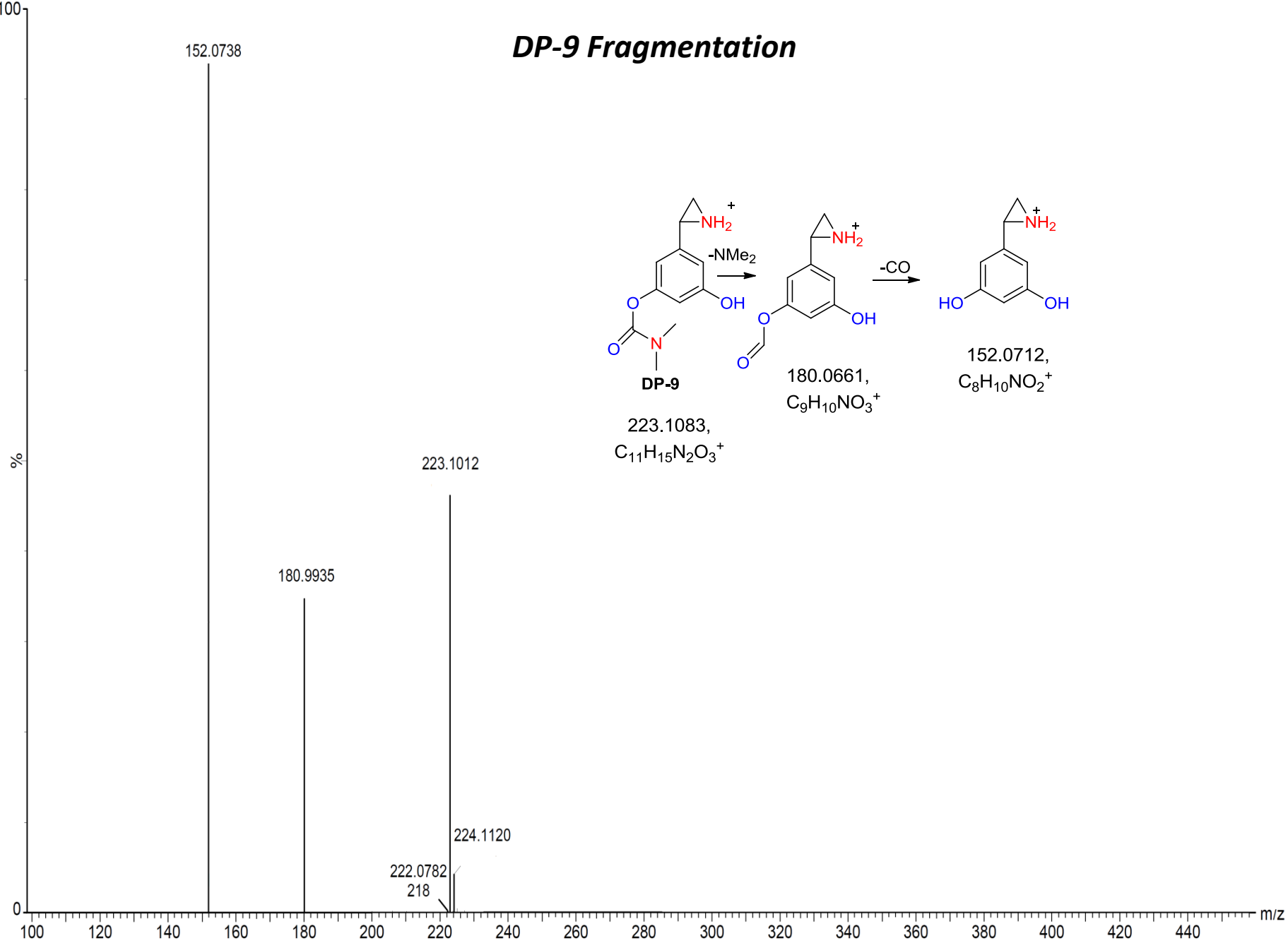
Figure 26: Fragmentation pattern and LCMS spectra of DP-9
