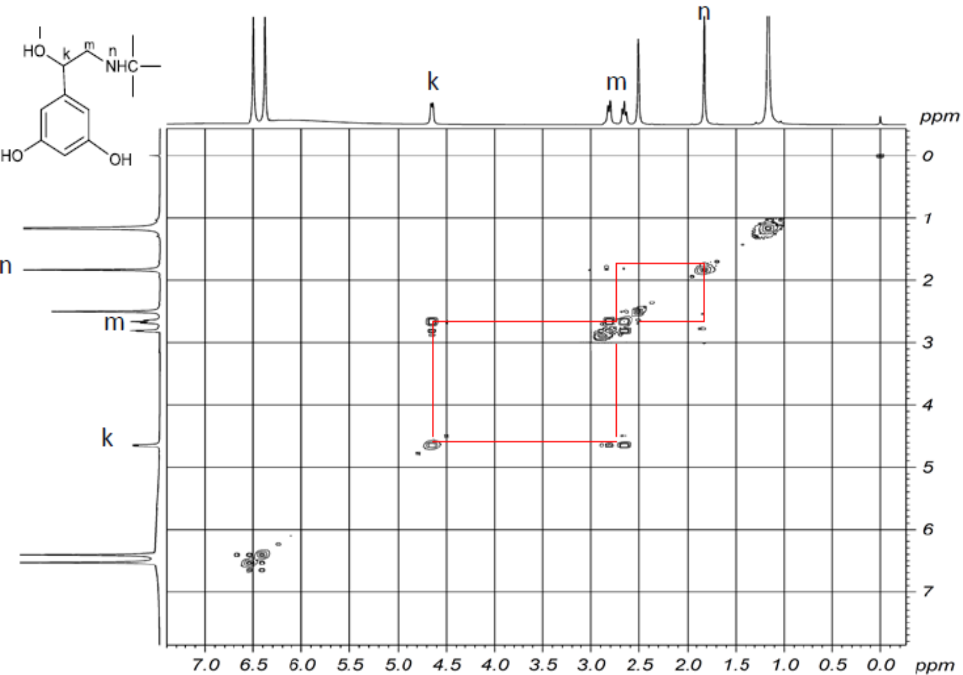
Figure 11: COSY NMR spectra of DP-3
