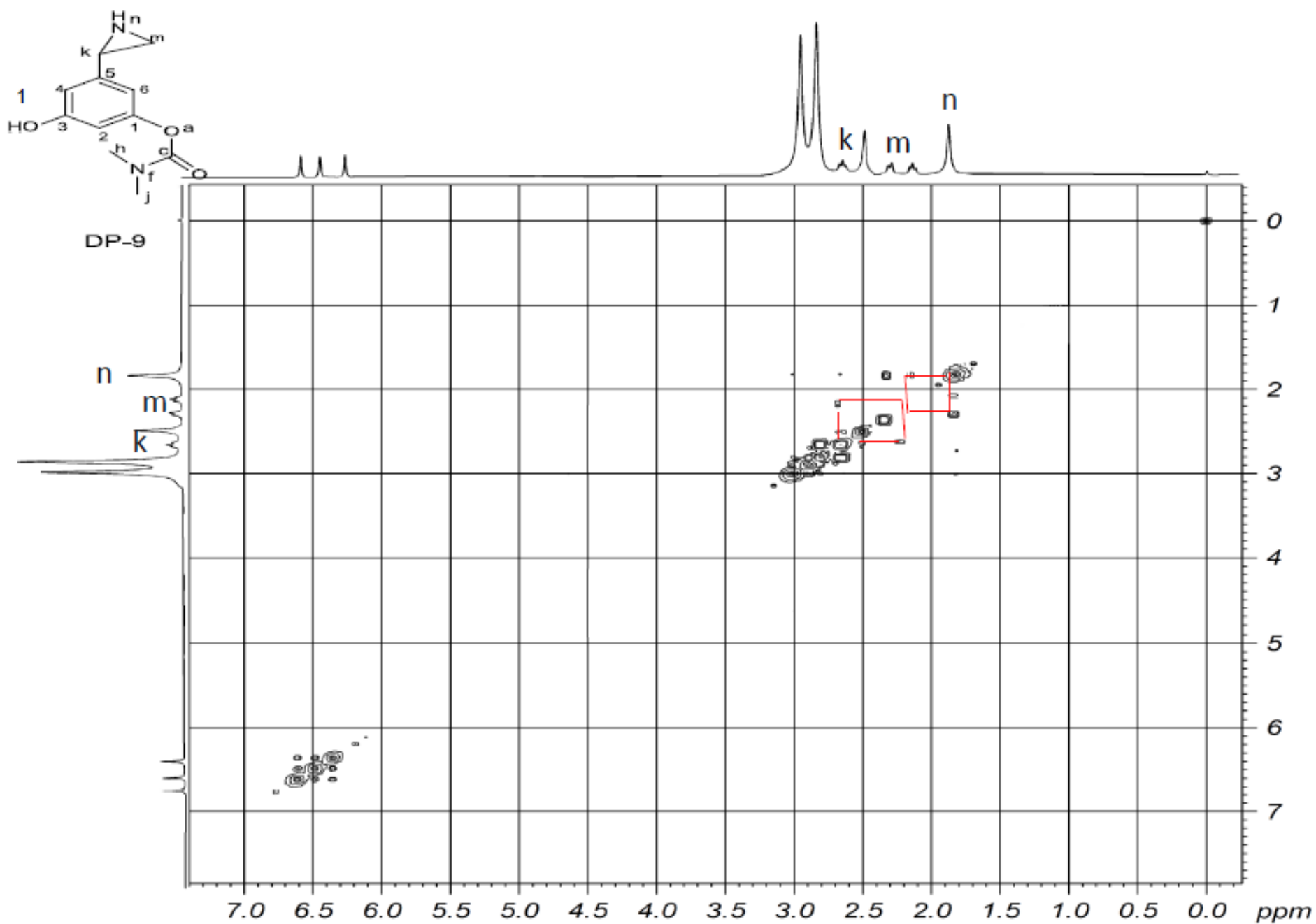
Figure 25: COSY spectra of DP-9
