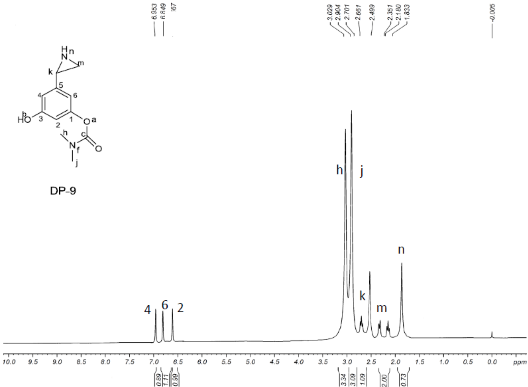
Figure 23: 1 H NMR spectra of DP-9
