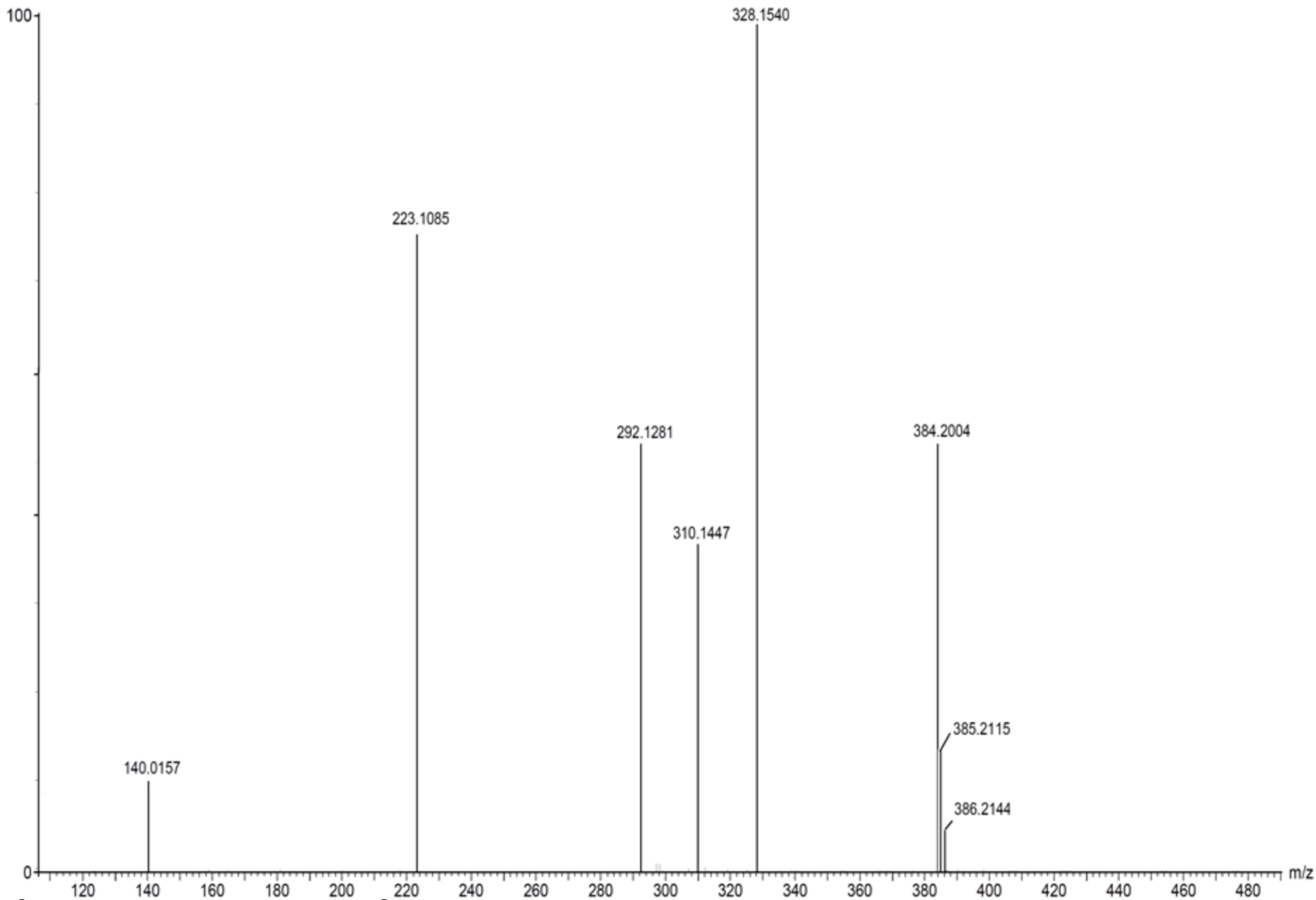
Figure 18: LCMS spectra of DP-5
