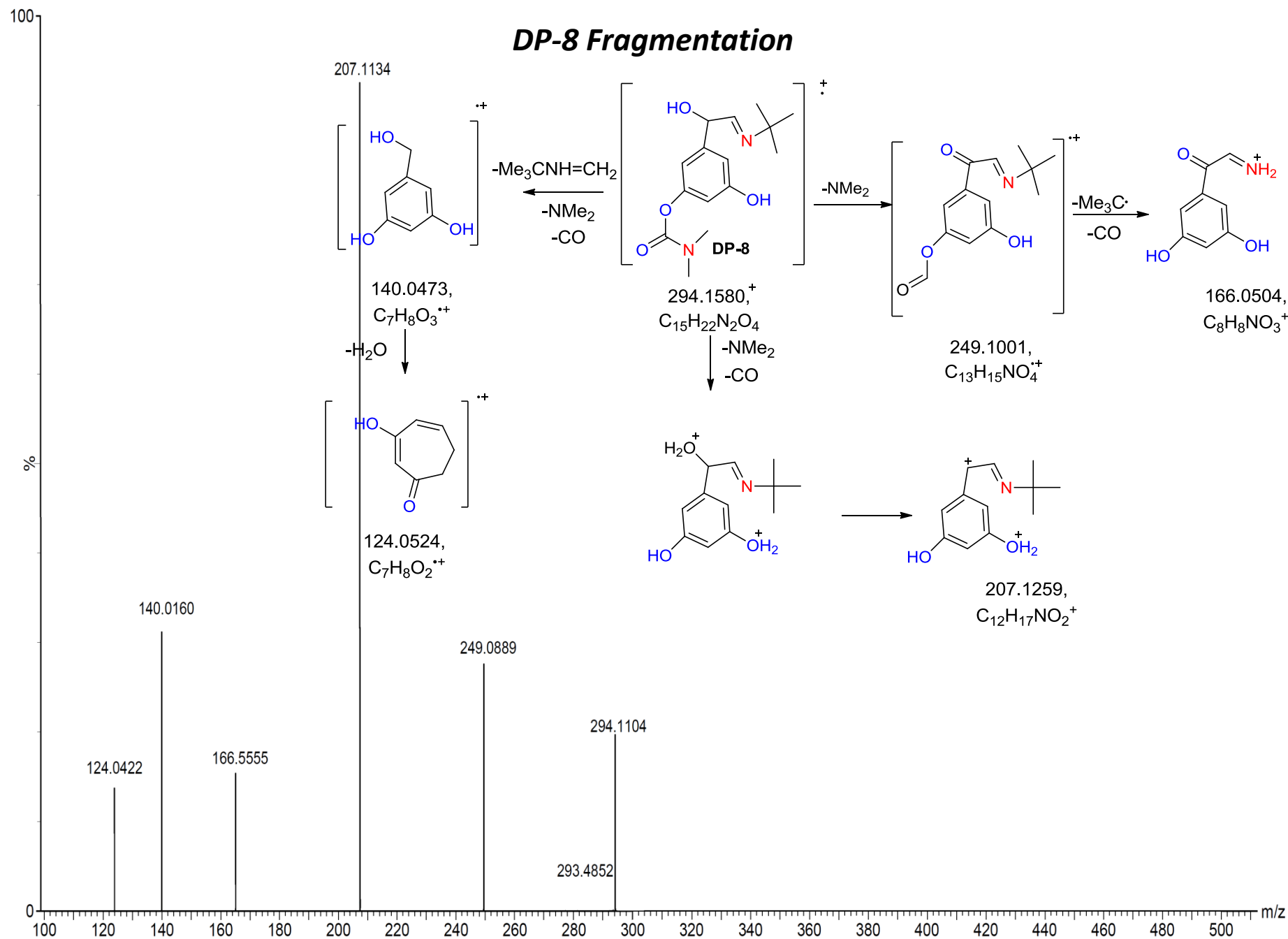
Figure 22: Fragmentation pattern and LCMS spectra of DP-8
