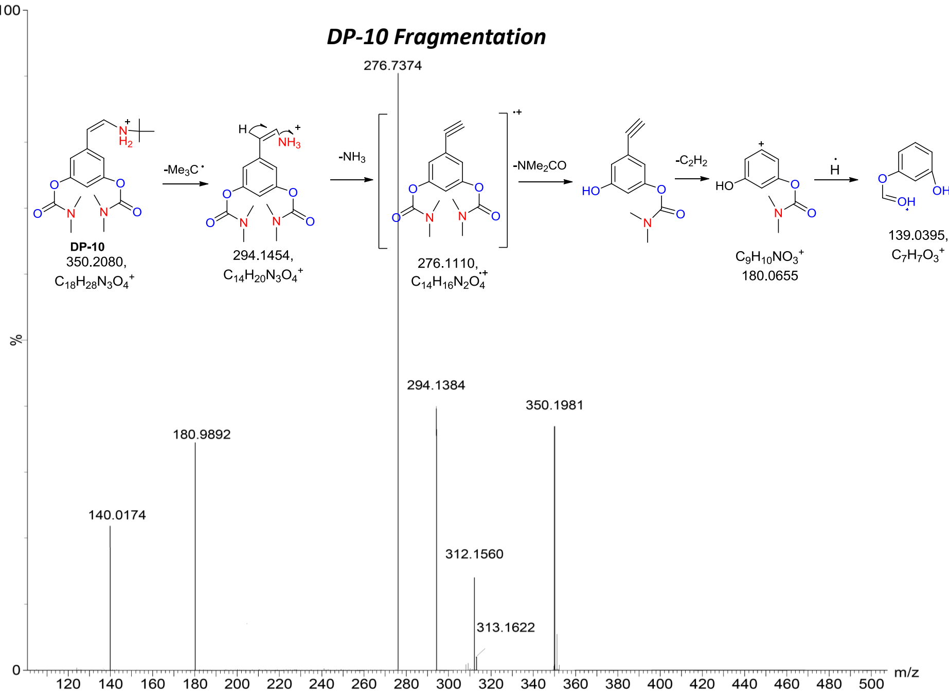
Figure 27: Fragmentation pattern and LCMS spectra of DP-10
