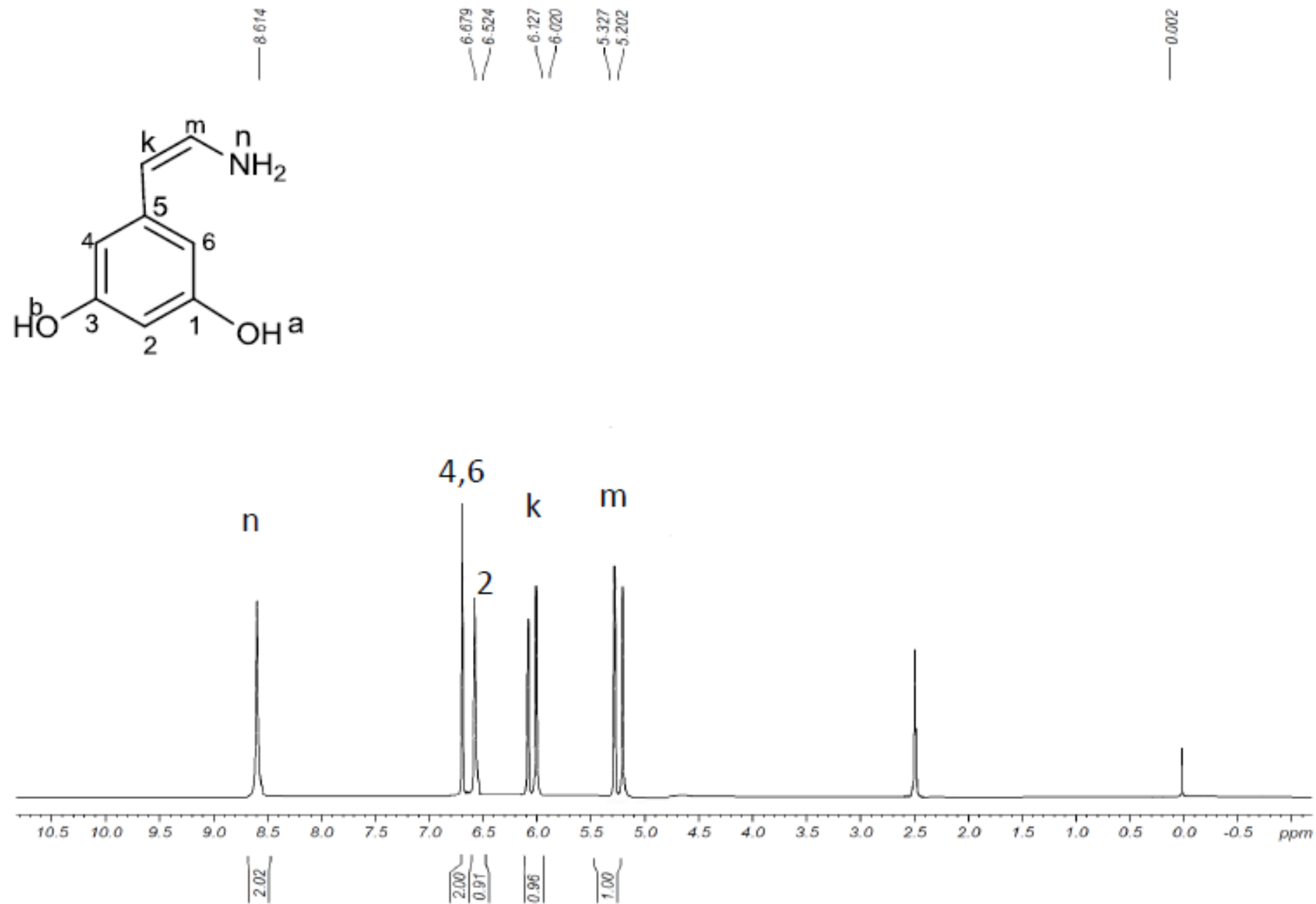
Figure 3: ^1\text{H} NMR spectra of DP-1
