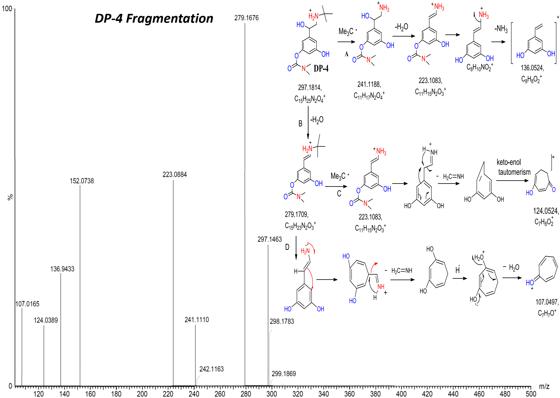
Figure 17: Fragmentation pattern and LCMS spectra of DP-4
