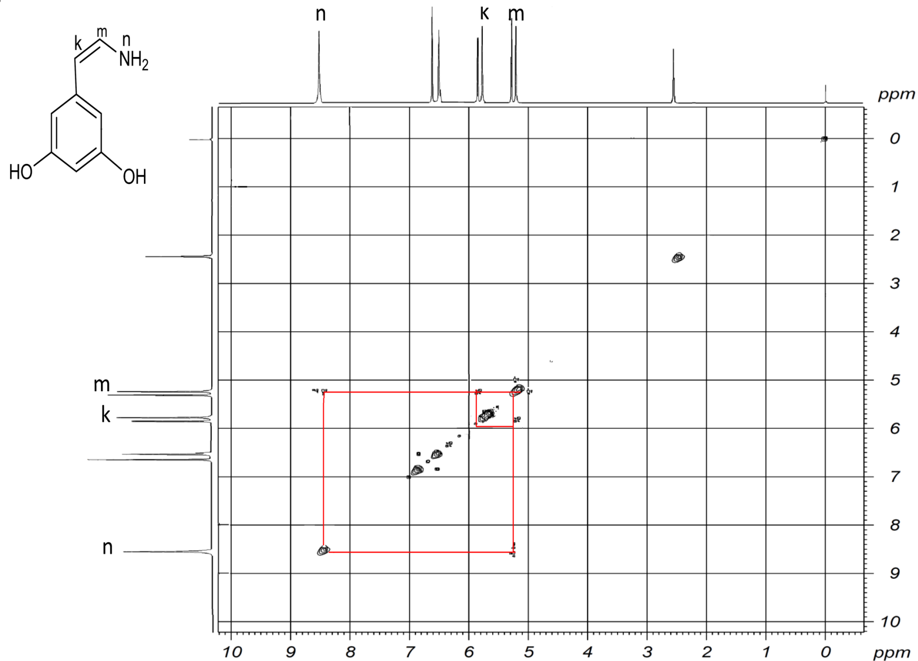
Figure 5: COSY NMR spectra of DP-1
