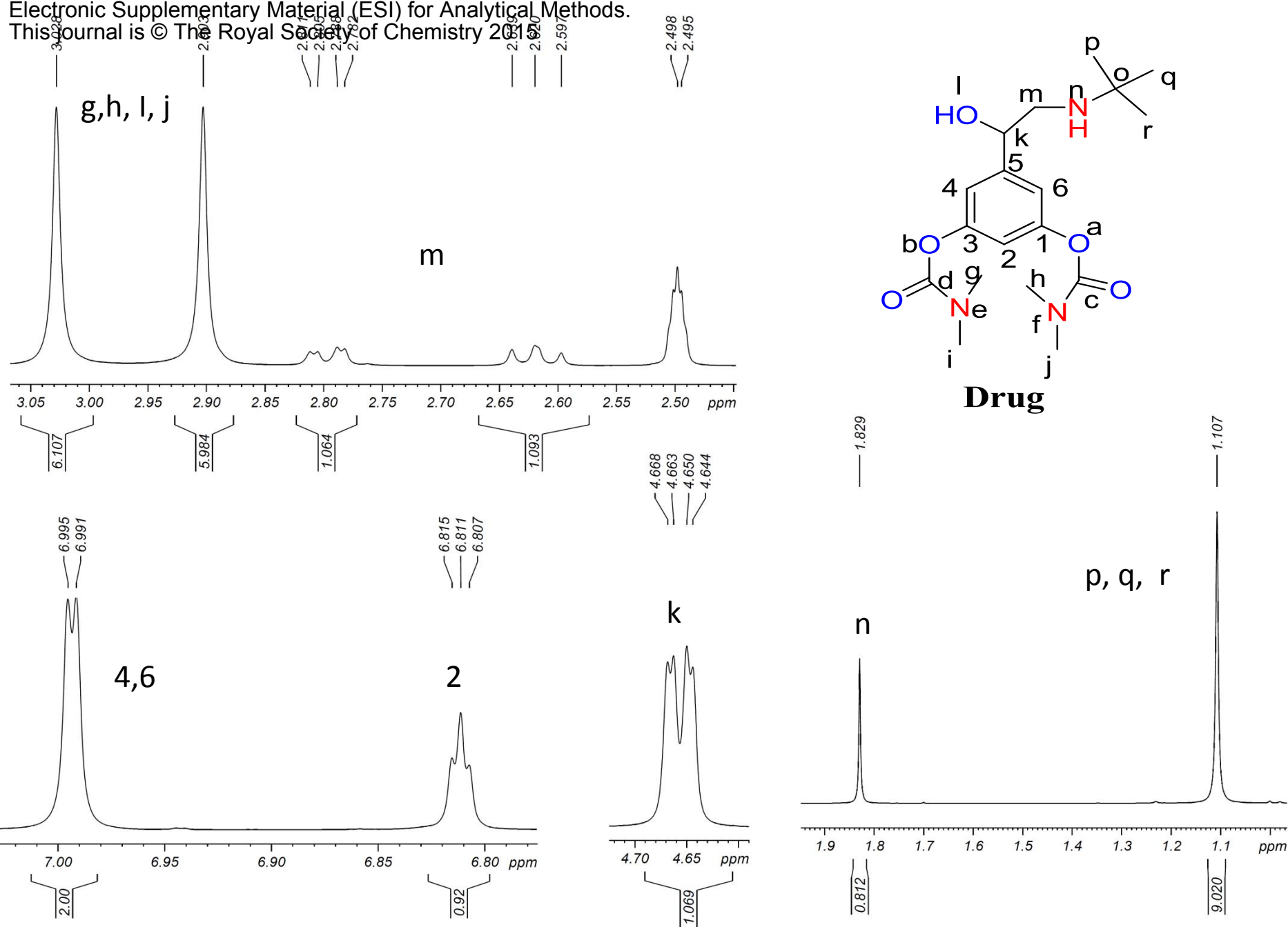
Sfigure 1: Expanded ^1\text{H} NMR spectra of Bambuterol
