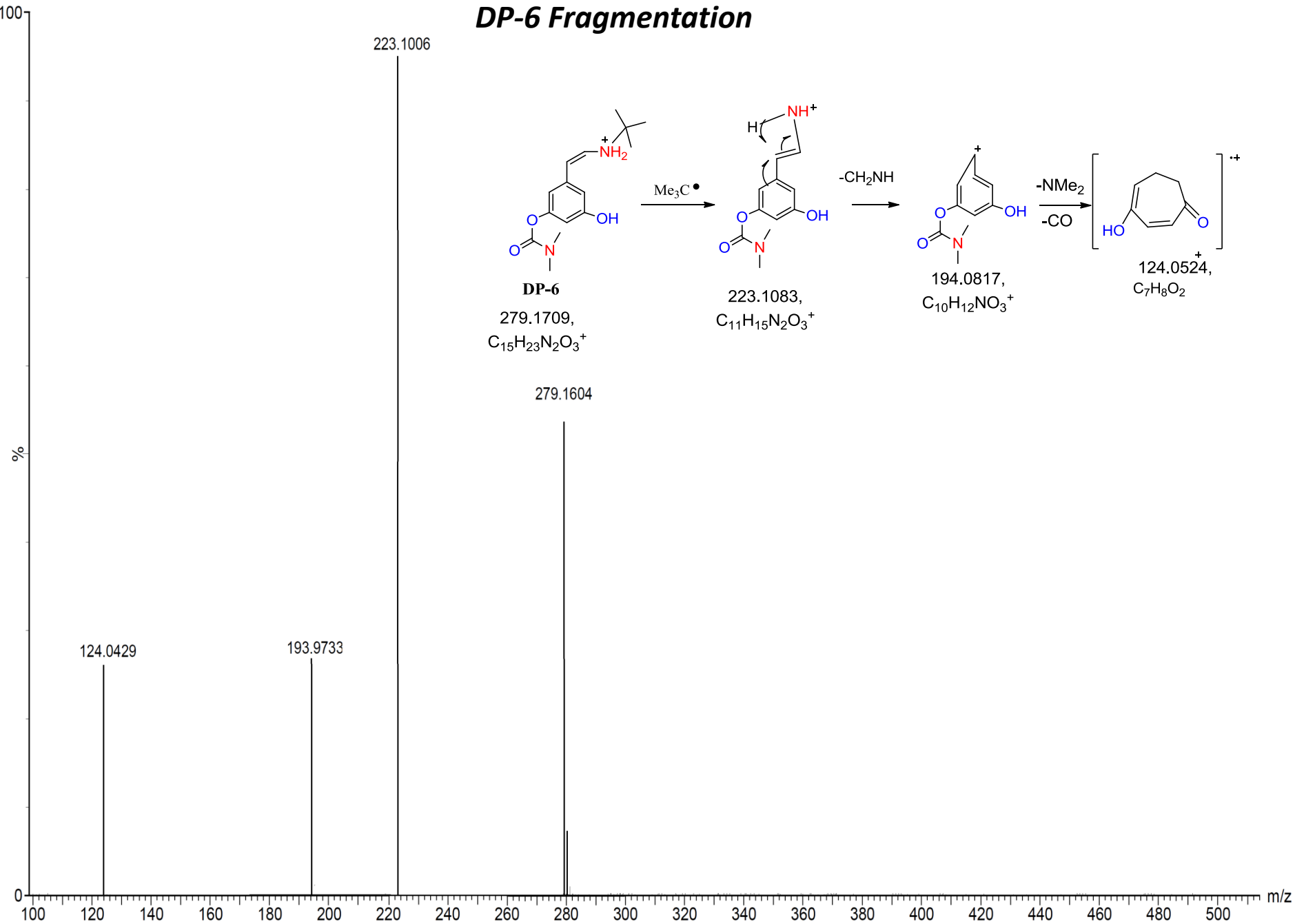
Figure 20: Fragmentation pattern and LCMS spectra of DP-6
