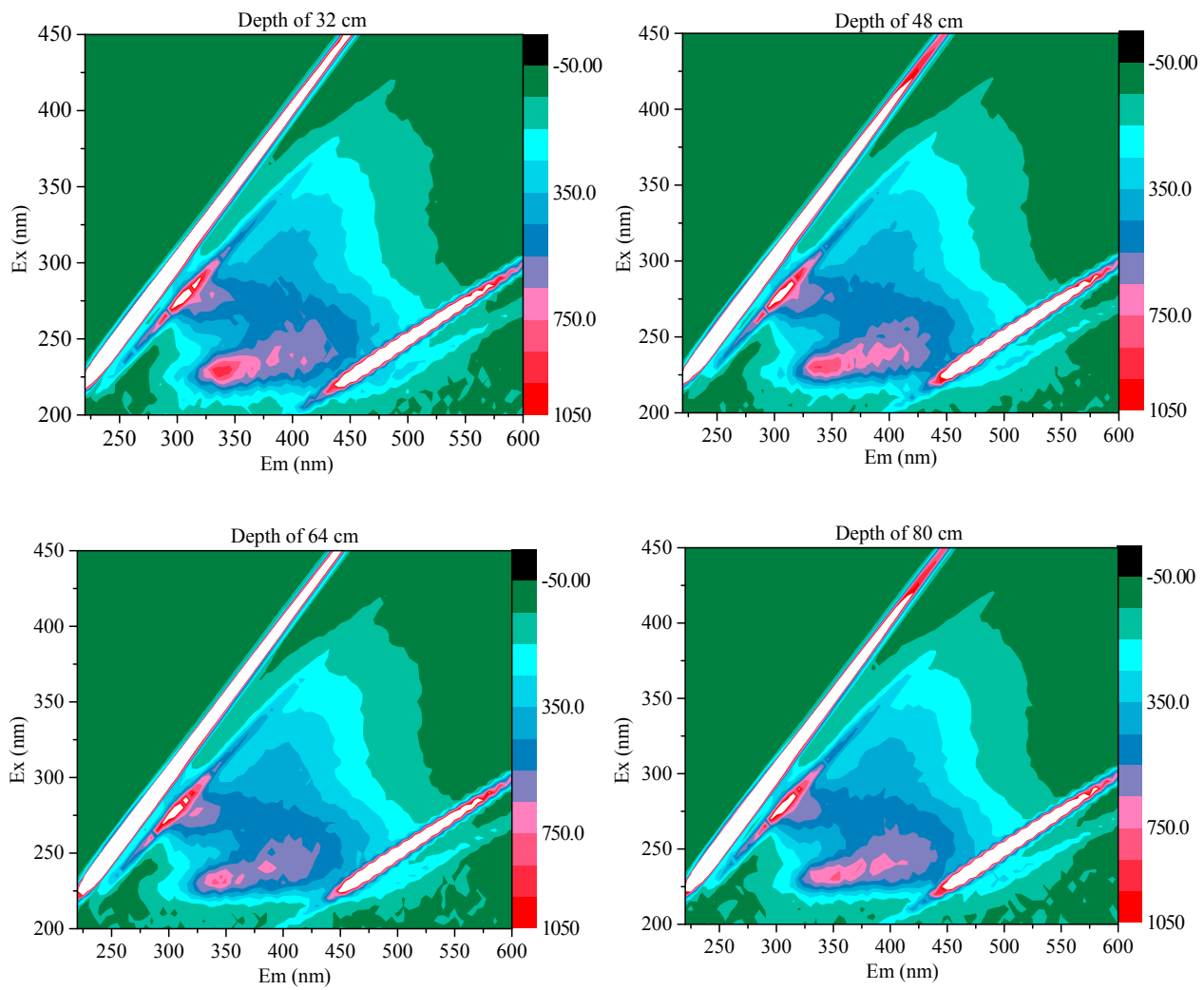
Fig. 1 EEM fluorescence spectra of DOC and DON at different media depth of BAF: (a) Samples taken on May 30 th ; (b) Samples taken on June 5 th ; (c) Samples taken on June 9 th
