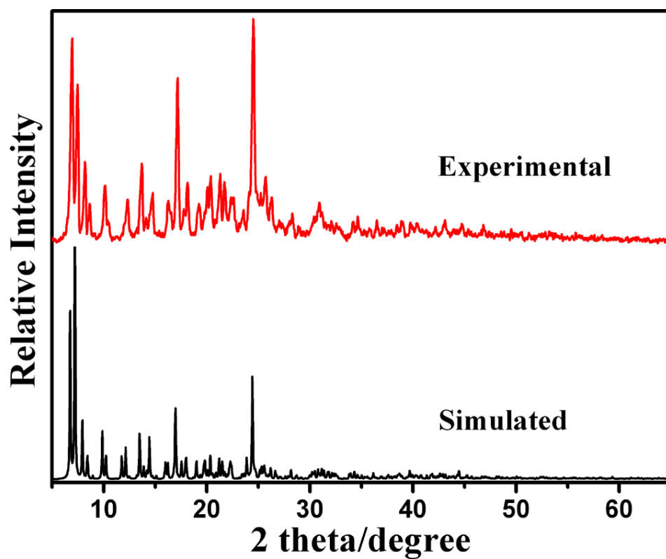
Fig. S1. The PXR D pattern of 1 is comparable to the simulated from the single crystal X-ray data.
