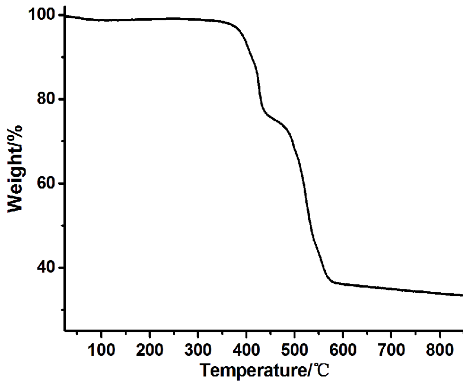
Fig. S2. Thermogravimetric curve of the title compound 1.
