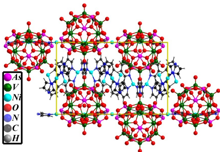
Fig. s1 packing structure of compound 1.
