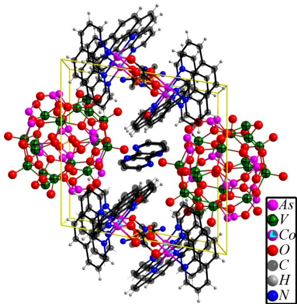
Fig. s6 packing structure of compound 6.
