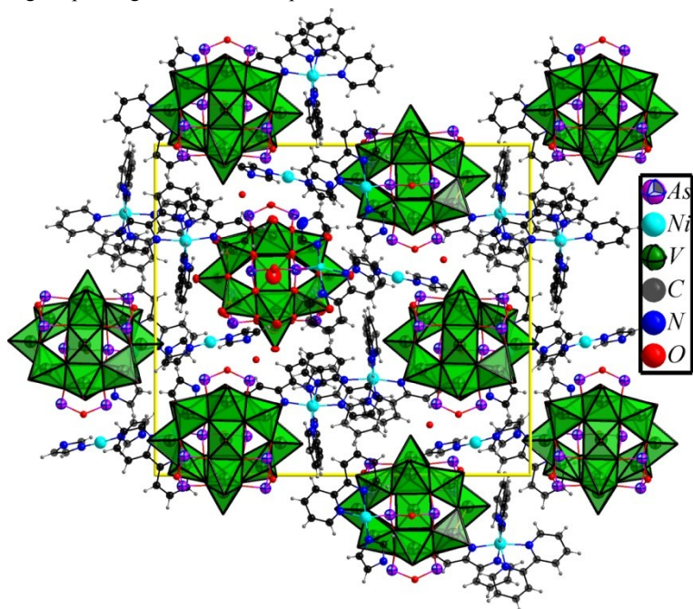
Fig. s2 packing structure of compound 1a.
