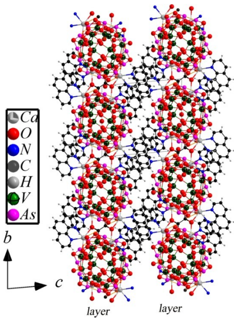
Fig. s5 packing structure of compound 5.
