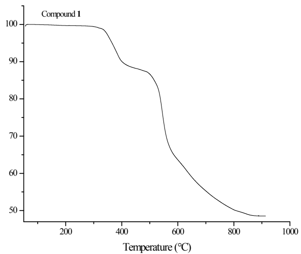
Fig. s10 TG curve of compound 1.
