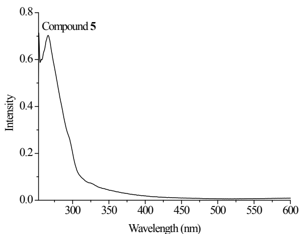
Fig. s9 UV-Vis spectra of compounds 1-6.
