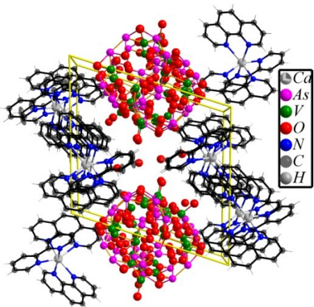
Fig. s4 packing structure of compound 4.
