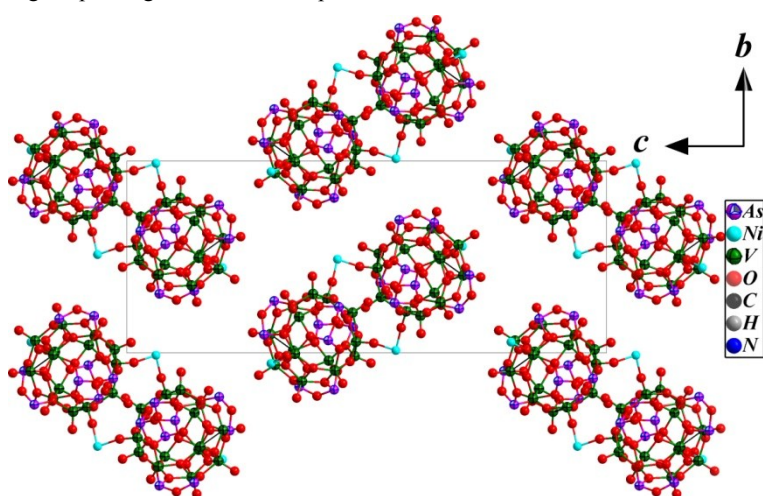
Fig. s3 packing structure of compound 2, carbons, nitrogens and hydrogens are omitted for clarity.
