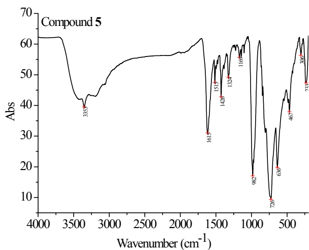
Fig. s7 IR spectra of compounds 1-6.
