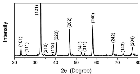
Figure S1 X-ray diffraction patterns of \text{La}_{0.875}\text{Ca}_{0.125}\text{FeO}_3 annealed at 800^\circ\text{C} .
