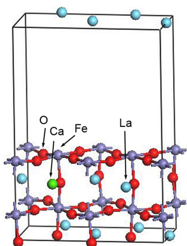
Figure S2 The optimized structure of \text{La}_{0.875}\text{Ca}_{0.125}\text{FeO}_3 (010) surface
