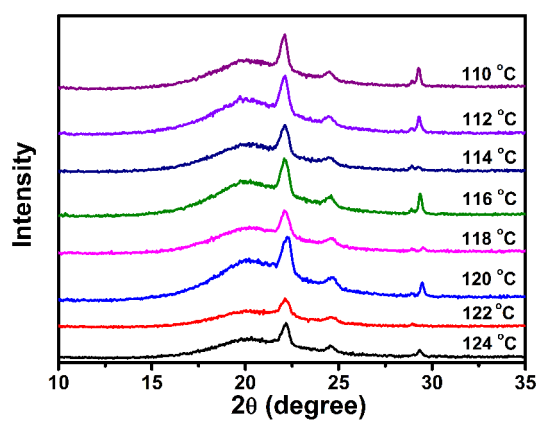
Figure S1. WAXD results of OBCs annealed at different temperatures.
