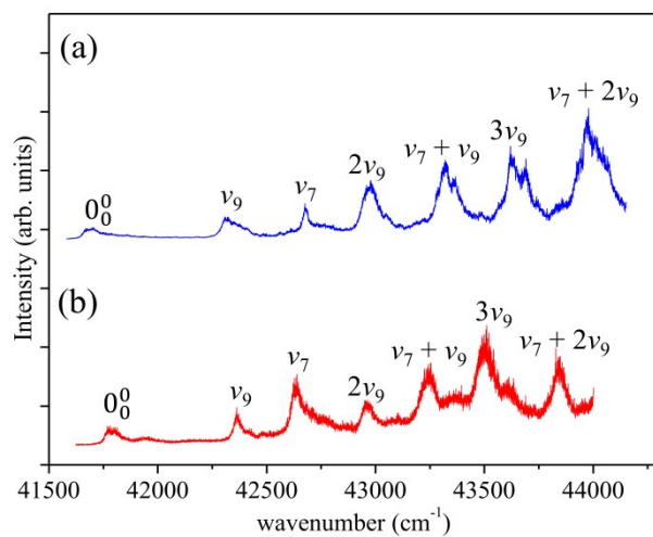
Fig. S1. Jet-cooled H photofragment action spectra obtained in predissociation of (a) methylamine and (b) methylamine- d_3 , taken from Refs. 24 and 25, respectively. The assignment of the observed bands is based on Ref. 14.
