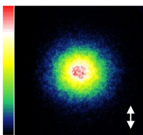
Fig. S2. Measured TCRD velocity map of the D photofragments, obtained from C–D bond breaking in methylamine- d_3 , following excitation to the 0_0^0 state.
