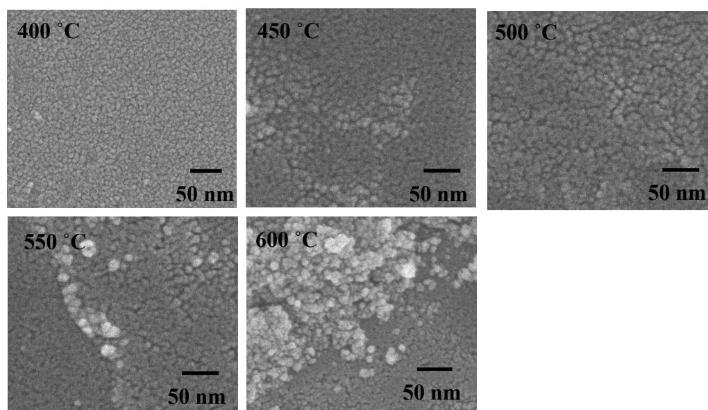
Fig. S1 The SEM images of TiO 2 nanoparticles with different calcined temperatures.
