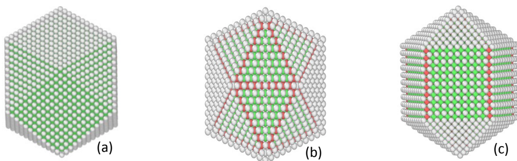
Figure: Cuboctahedron (a), Icosahedron (b) and Decahedron (c) Au cluster. FCC atoms are colored green, HCP red and other atoms are colored white
