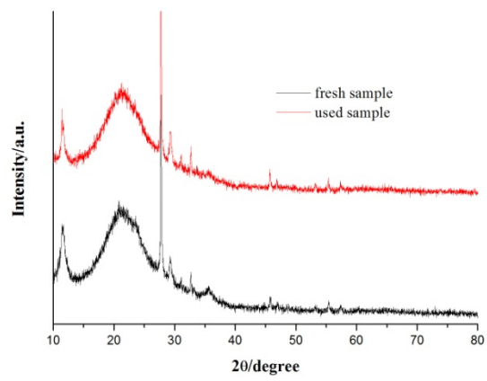
Fig. S3. The XRD patterns of the fresh and used samples.
