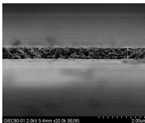
Fig. S1. The cross-section SEM of meso -SiO 2 /Cu-Bi 2 O 3 film.
