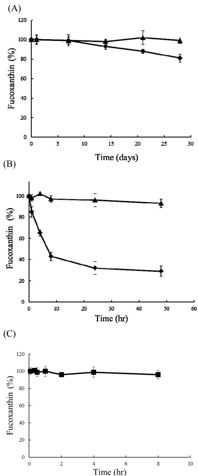
Fig S. Effect of temperature on fucoxanthin degradation. Fucoxanthin standard (◆) and high stability fucoxanthin (HS-Fx, ▲ or ■) were incubated on -20^{\circ}\text{C} (A), 4^{\circ}\text{C} (B) and room temperature (C) for indicated time. Fucoxanthin content was examined by HPLC. Data were from three independent experiments.
