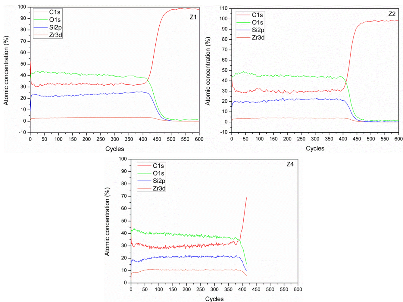
Fig S11 XPS profiles on PC-Z1, PC-Z2 and PC-Z4
