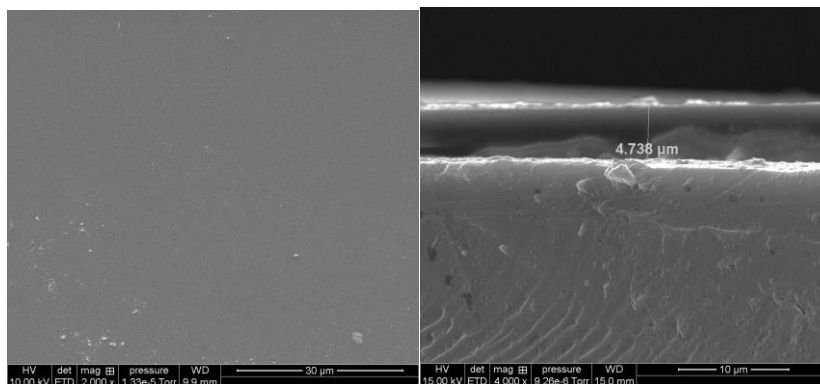
Fig S12: SEM images recorded on PC-Z4 sample, (a) surface and (b) cross section
