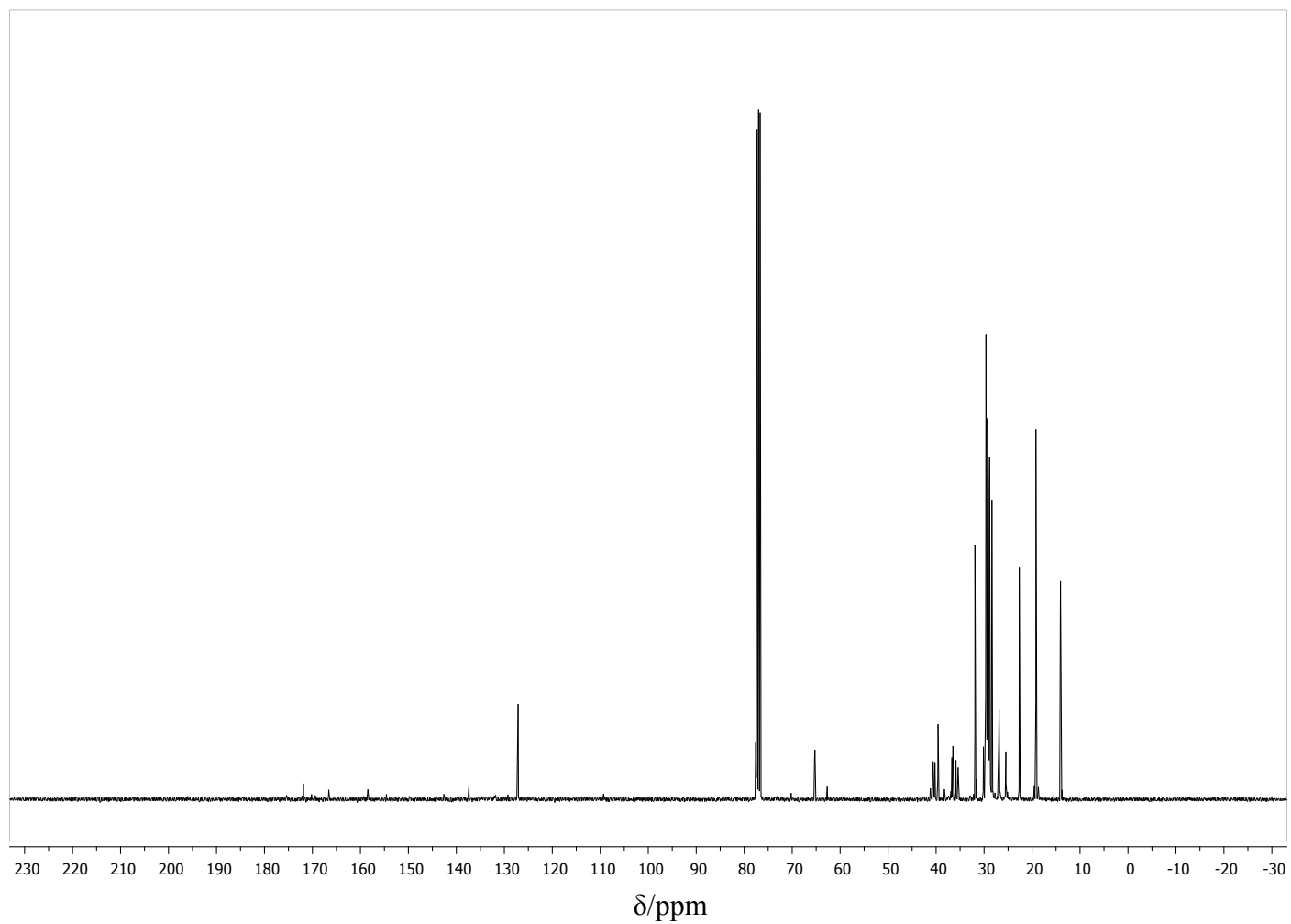
^{13}\text{C} -NMR spectrum of compound Zn-4 .
