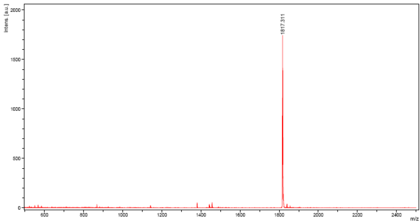
Mass spectrum of compound 4
