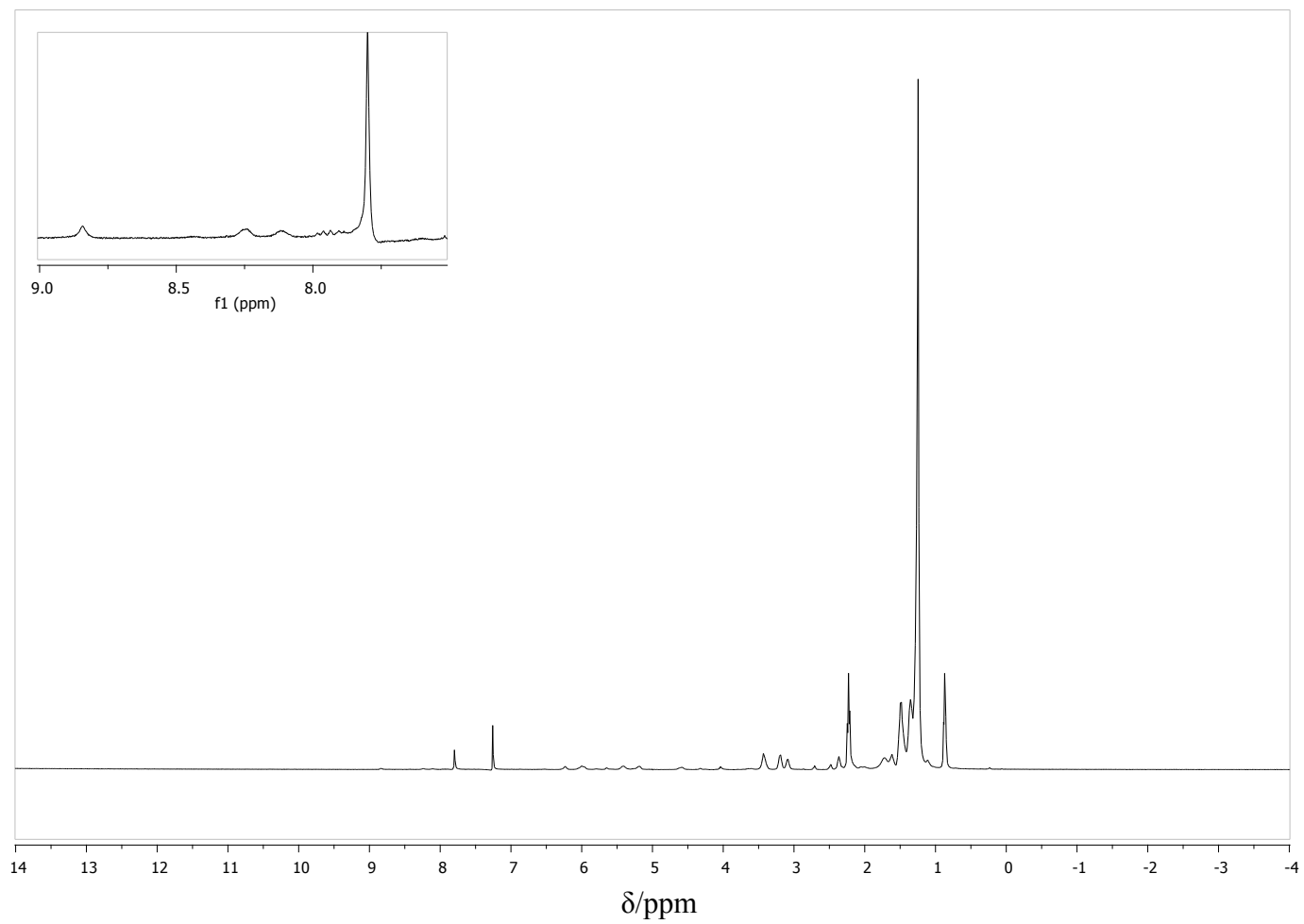
^1\text{H-NMR} spectrum of compound Zn-4
