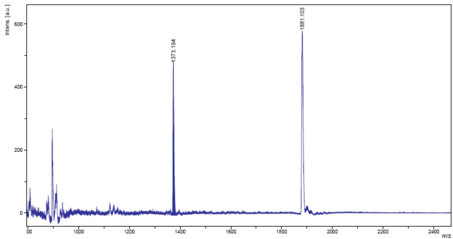
Mass spectrum of compound Zn-4
