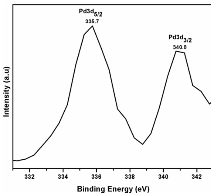
Fig. S1: XPS spectra of spent catalyst
