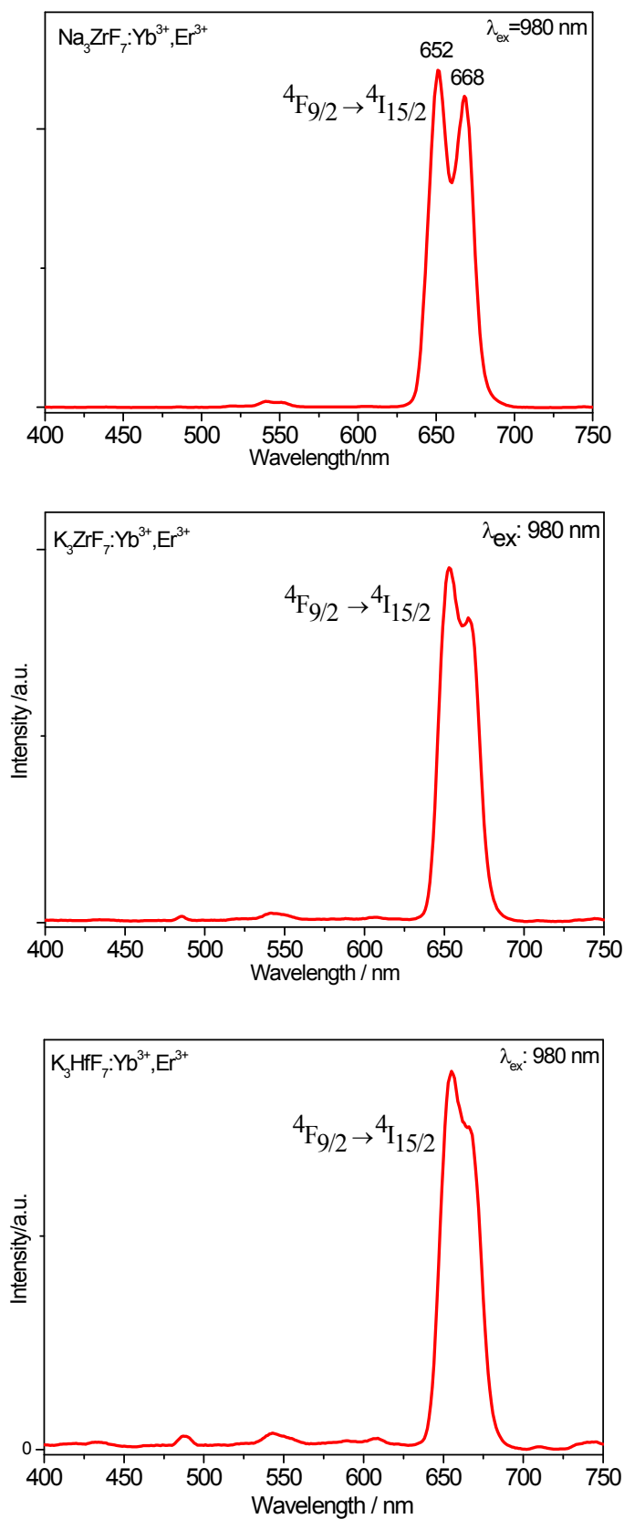
Figure S2 Up-conversion emission spectra of A_3MF_7:Yb^{3+},Er^{3+} (20/2 mol%) (A=Na, K, M = Zr, Hf) NCs
