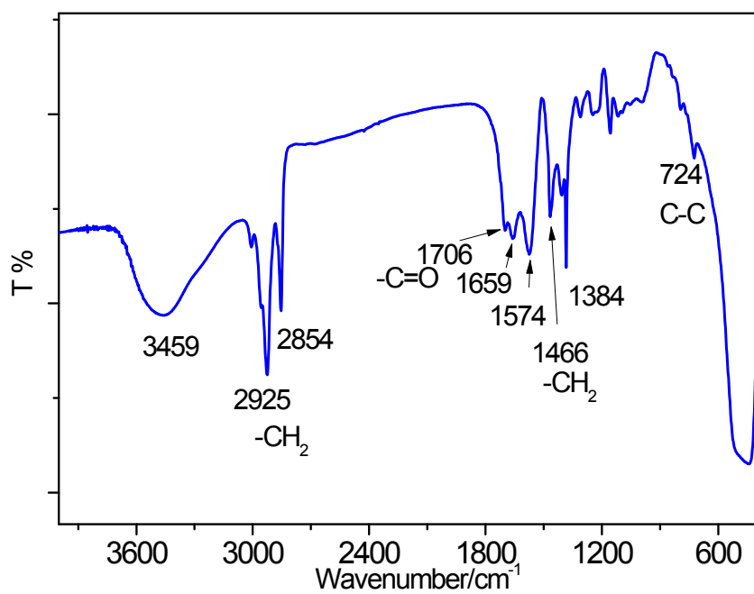
Figure S1 FT-IR spectrum of as-obtained K_3ZrF_7:Eu^{3+} sample
