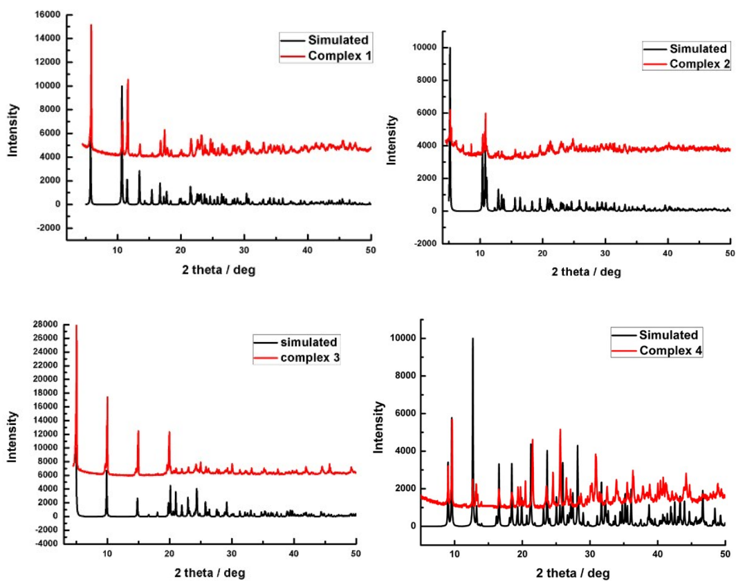
Figure S11. X-ray Powder Diffraction Analyses.
