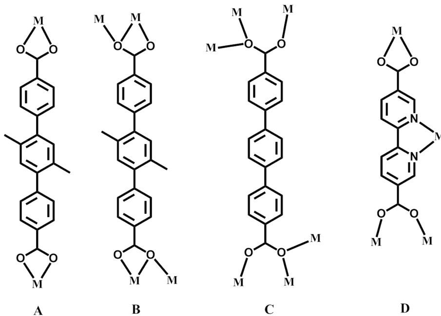
Figure S13. Coordination mode of ligands in 1-4.
