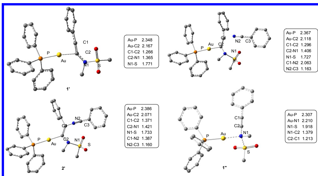
Fig. S3. Structures of intermediates 1' , \text{TS}1'-2' , 2' shown in Fig. 2 and 1'' . The bond distances are given in Å.
