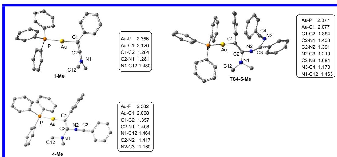
Fig. S4. Structures involved in Fig. 3 (b) where Me is attached on N1 atom. The bond distances are given in Å.
