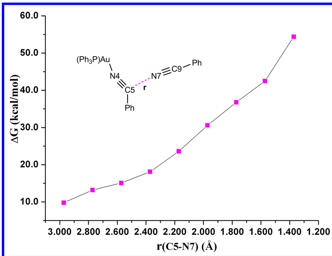
Fig. S2. Gibbs free energy changes with the second nitrile approaching to the C5 atom of the Au-nitrile species. The C5...N7 shortening goes with a decrement of 0.2 Å.
