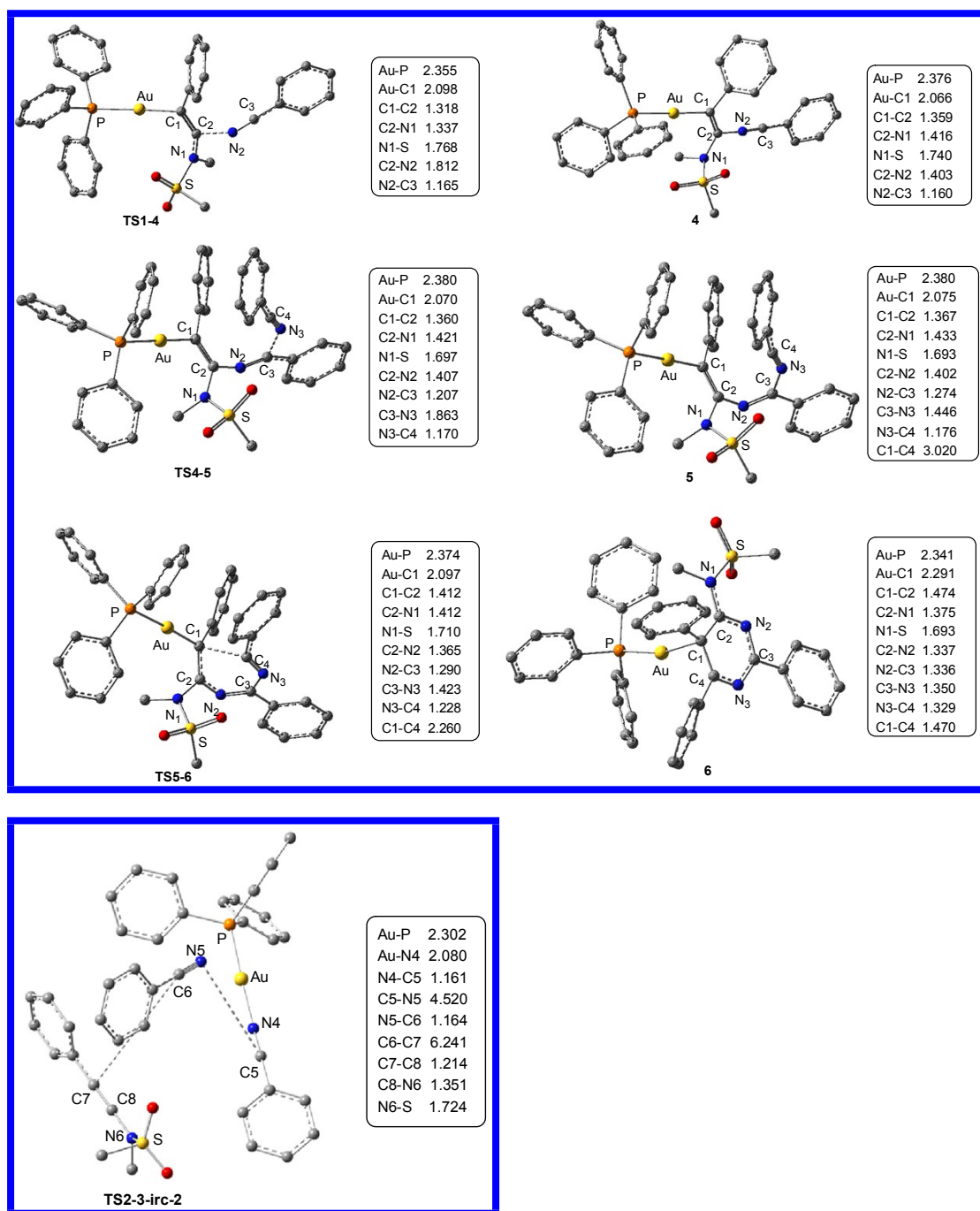
Fig. S1. Structures involved in path a \ path b and path c and TS2-3-irc-2. The bond distances are given in Å.
