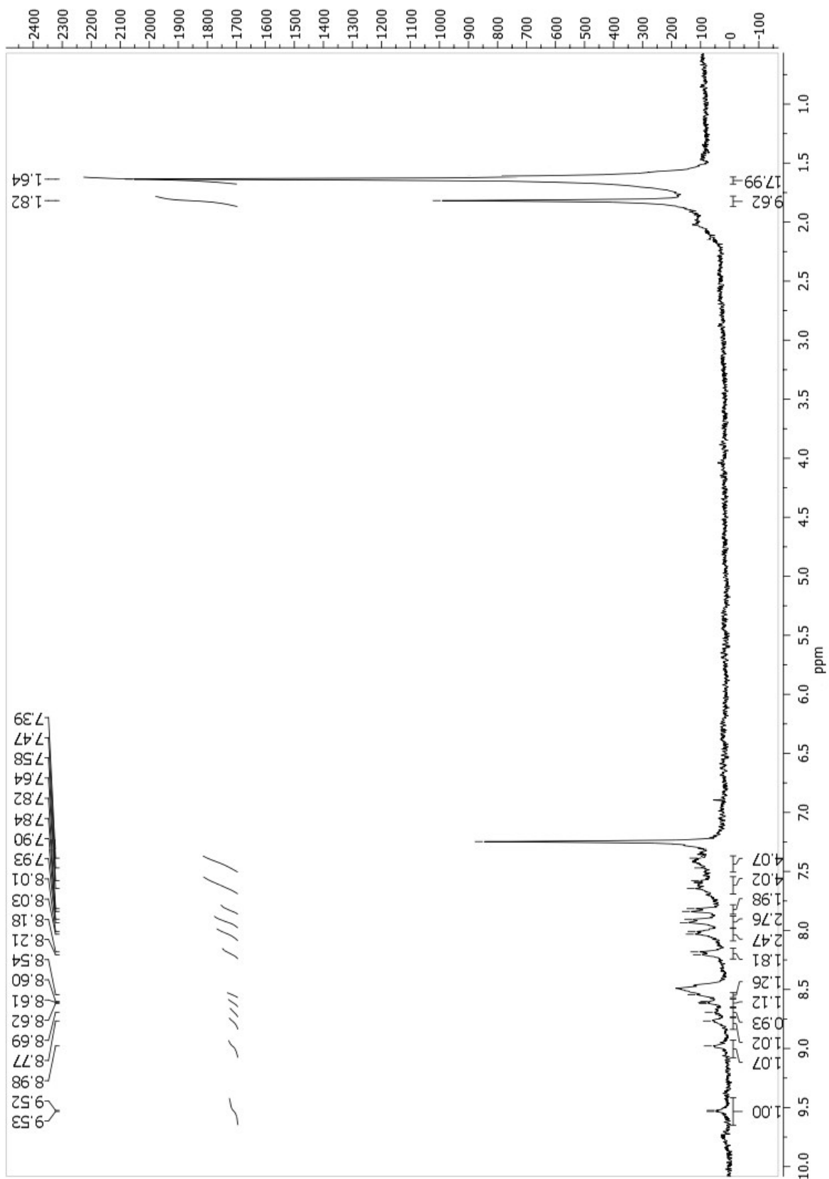
Figure S10: ^1\text{H} NMR spectrum of 2,3-[1'-2'-phenanthrene(b)pyrazino]-5,10,15-tris(4- tert -butylphenyl)corrole ( 8 )
