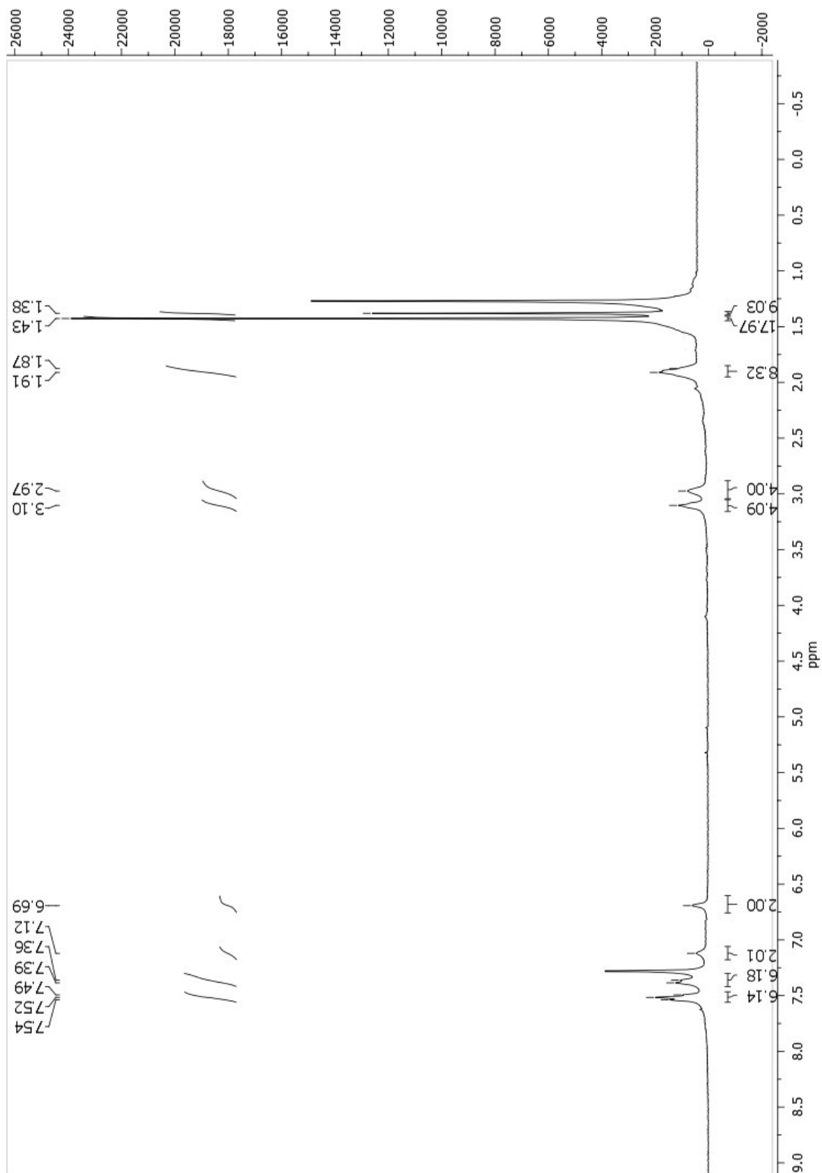
Figure S6: 1 H NMR spectrum of 2,3,17,18-bis[1'-2'-cyclohexane(b)pyrazino]-5,10,15-tris(4-tert-butylphenyl)corrolato-Cu ( 6 )
