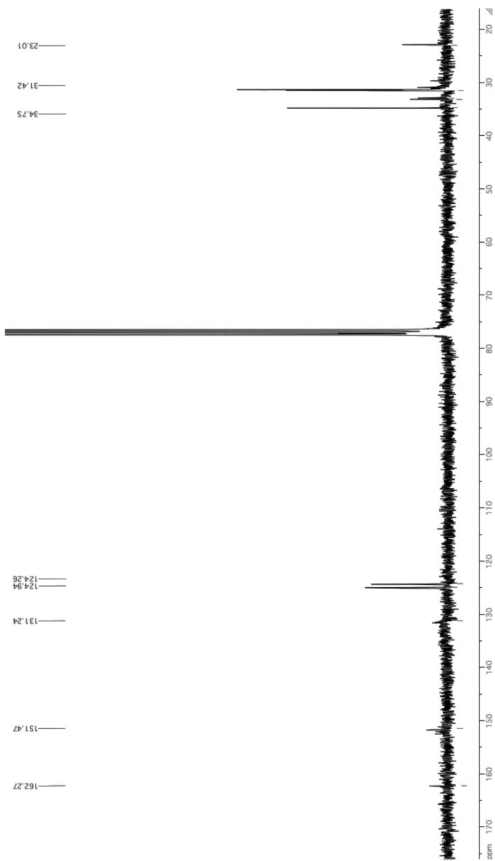
Figure S2: ^{13}\text{C} NMR spectrum of 2,3-[1'-2'-cyclohexane(b)pyrazino]-5,10,15-tris(4- tert -butylphenyl)corrolato-Cu ( 4 )
