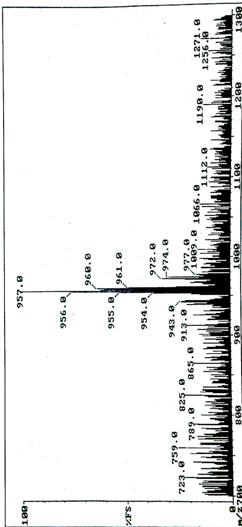
Figure S5: FAB spectrum of 2,3-[1'-2'-phenanthrene(b)pyrazino]-5,10,15-tris(4- tert -butylphenyl)corrolato-Cu (5)
