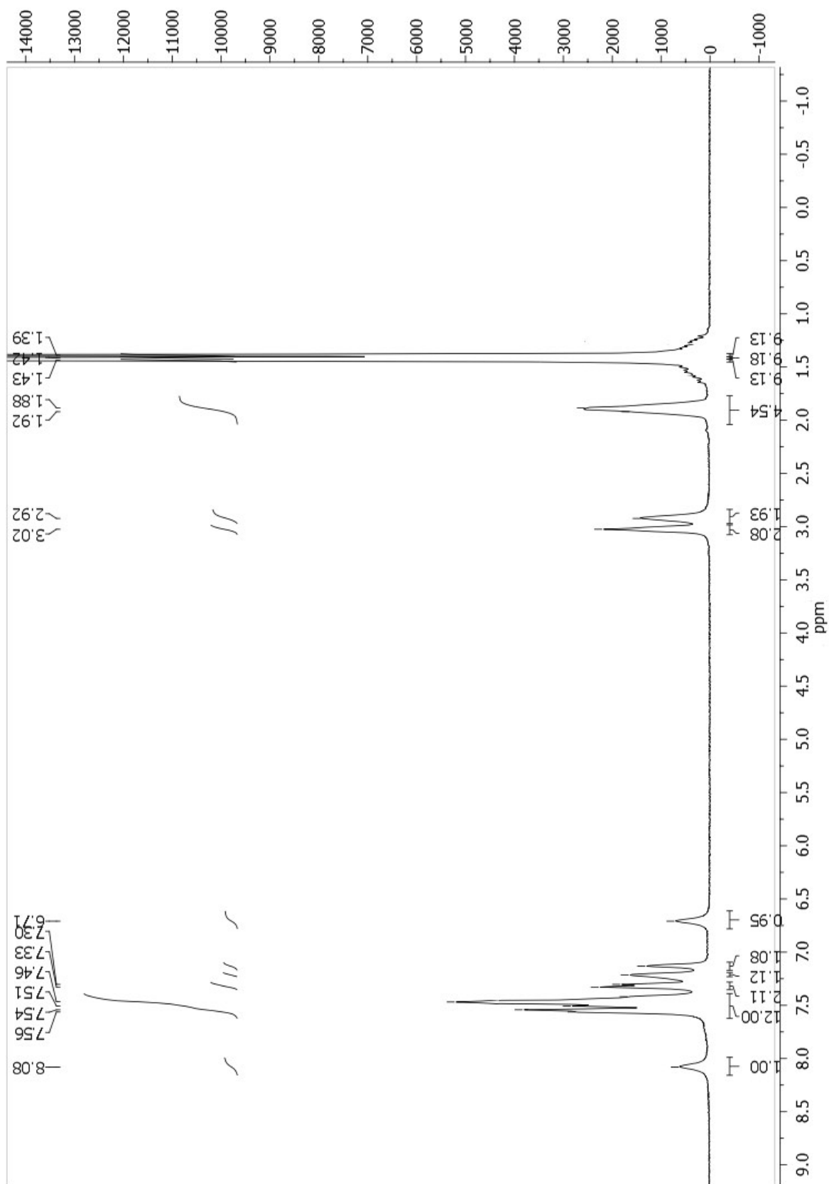
Figure S1: 1 H NMR spectrum of 2,3-[1'-2'-cyclohexane(b)pyrazino]-5,10,15-tris(4- tert -butylphenyl)corrolato-Cu ( 4 )
