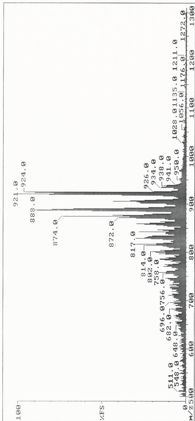
Figure S9: FAB spectrum of 2,3-[1'-2'-cyclohexane(b)pyrazino]-17-NO 2 -18-NH 2 -5,10,15-tris(4- tert -butylphenyl)corrolato-Cu (7)
