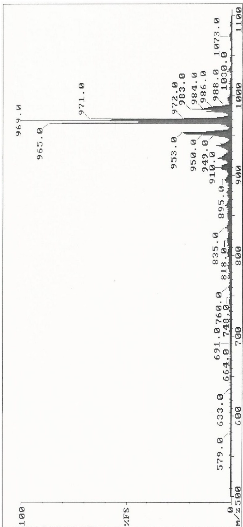
Figure S7: FAB spectrum of 2,3,17,18-bis[1'-2'-cyclohexane(b)pyrazino]-5,10,15-tris(4- tert -butylphenyl)corrolato-Cu ( 6 )
