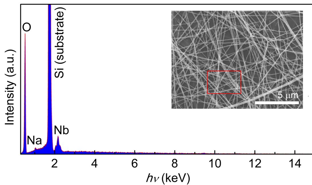
Fig. S1 The Energy dispersive spectrum (EDS) analysis result of the electrospun \text{NaNbO}_3 nanofibers. The inset picture shows the measured area of the sample. The result confirms that the nanofiber is consisted of pure Na, Nb and O elements.
