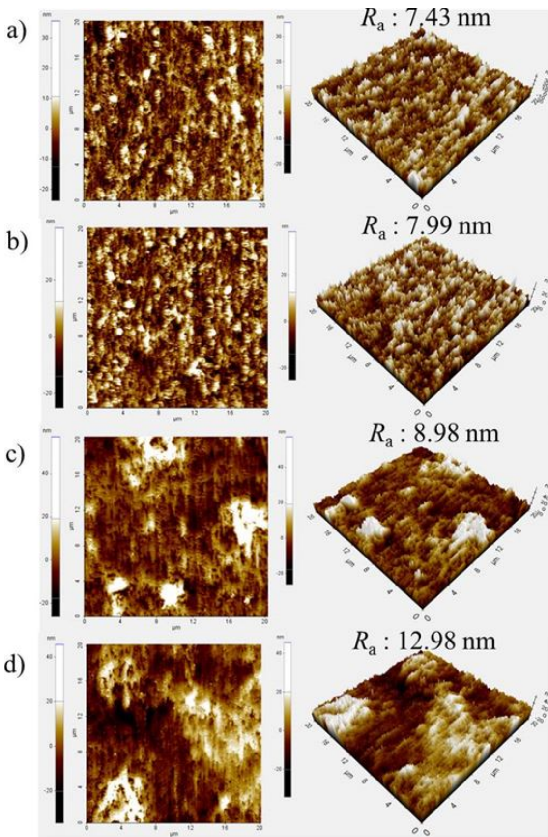
Figure S1. AFM images of the unrubbed cellulose film fabricated using a (a) 1 wt%, (2) 3 wt%, (3) 5 wt%, and (4) 10 wt% solution by spin coating (4000 rpm, 60 sec).
