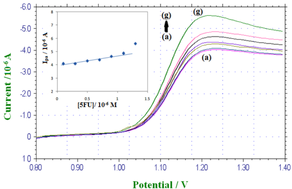
SI. Fig. 2. SCV of bare GCE in 5FU solution at different concentrations at (a) 0.1, (b) 0.3, (c) 0.5, (d) 0.7, (e) 0.9, (f) 1.1 and (g) 1.3 \times 10^{-6} M (Inset: Plot of the peak currents against concentrations of 5FU).
