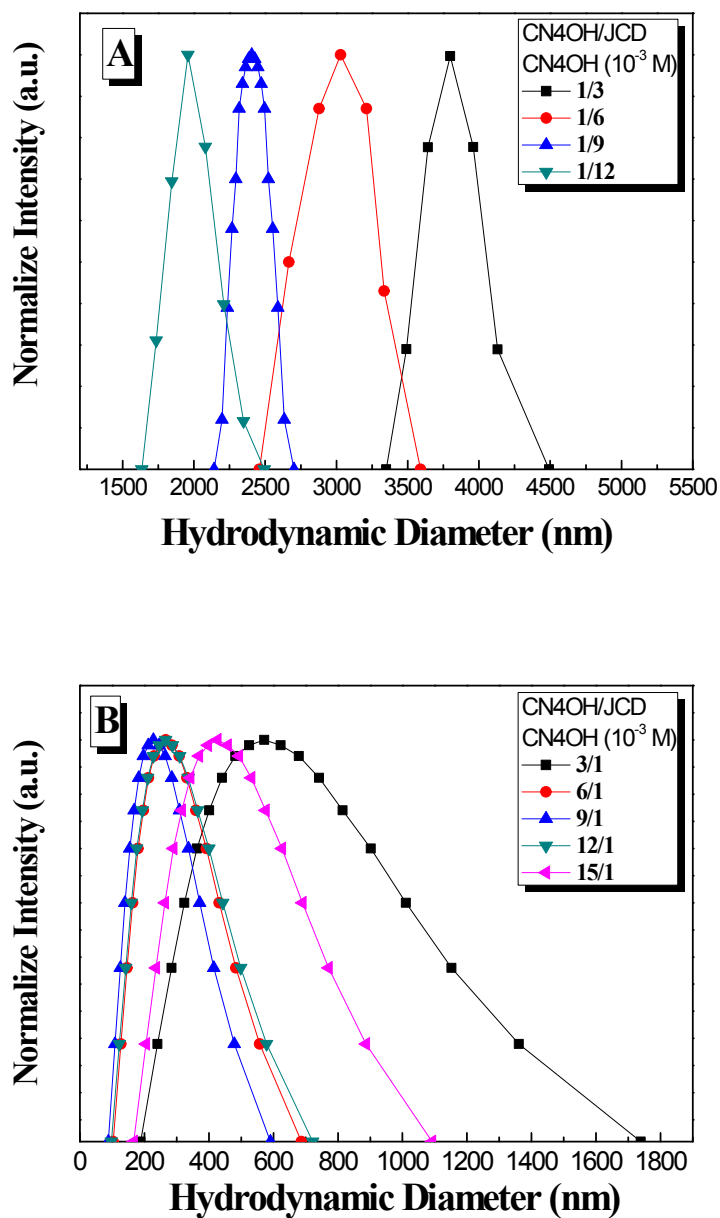
Figure S4 Hydrodynamic size histogram of CN4OH/JCD( x/y ) with (A) x/y < 1 and (B) x/y > 1 mixtures with a constant concentration of CN4OH ( = 10^{-3} M) in DMSO.
