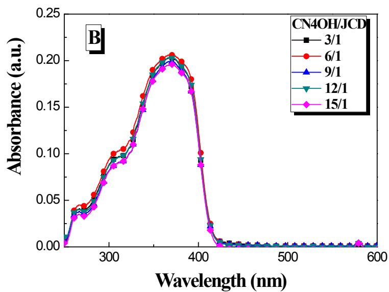
Figure S3 Solution absorption spectra of CN4OH/JCD( x/y ) with (A) x/y < 1 and (B) x/y > 1 mixtures with a constant concentration of CN4OH ( = 10^{-3} M) in DMSO.
