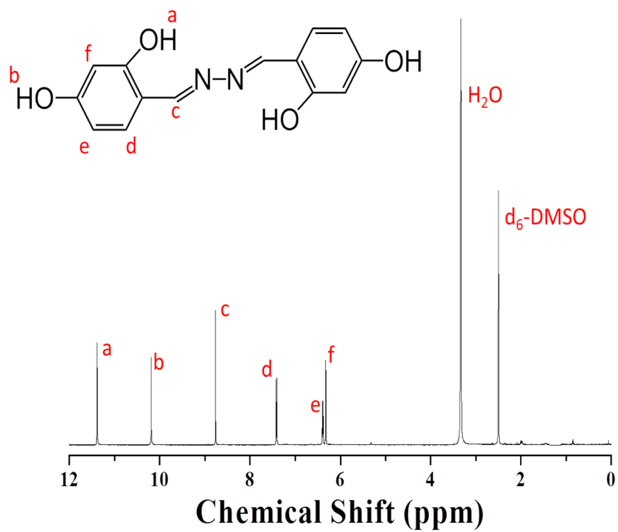
Figure S2 1 H NMR spectra of CN4OH (10 -3 M) (d 6 -DMSO).
