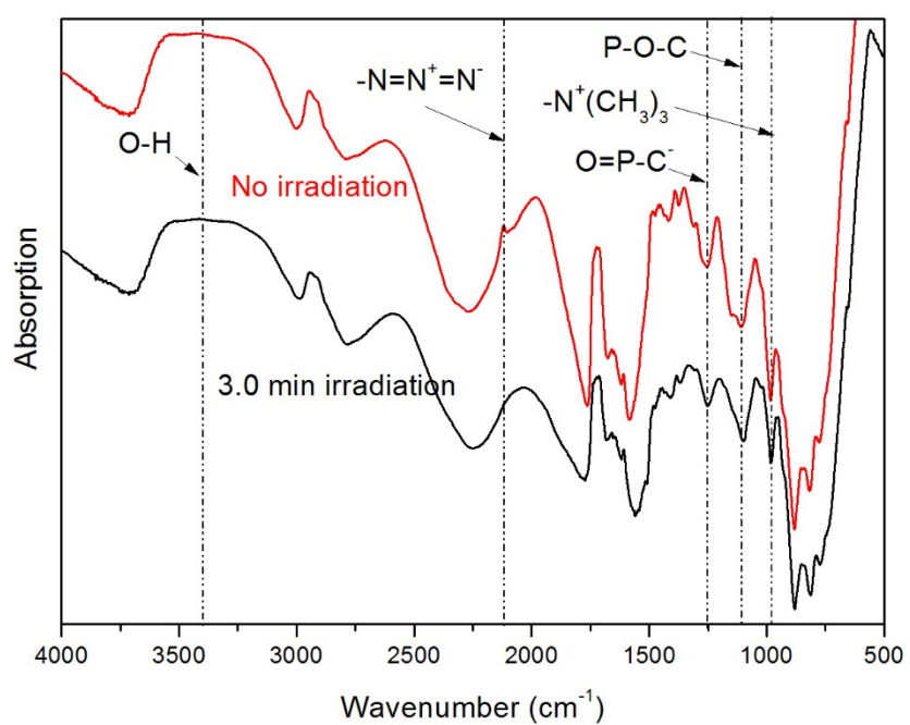
Figure S1. FT-IR reflection absorption spectra of PMBV/AWP multilayer hydrogel membranes photocrosslinked by UV irradiation
