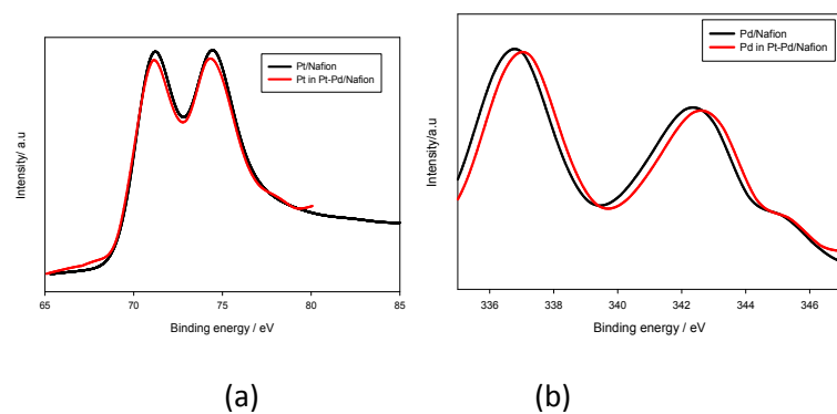
S2: Relative binding energy positions of (a) Pt(4f) and (b) Pd(3d) under monometallic and bimetallic forms
