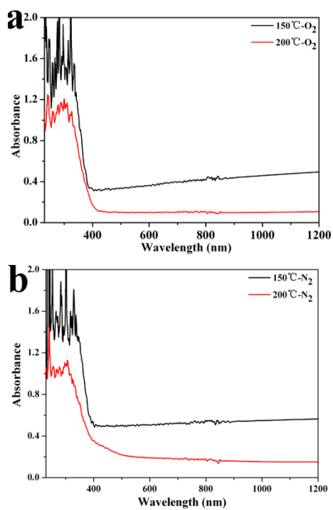
Figure S1 UV-vis diffuse reflection spectra of TiO 2-x nanowires (150 °C) and nanobelts (200 °C) calcinated in air (a) and in nitrogen (b)
