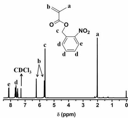
Fig. S1 1 H NMR spectrum of NBMA.
