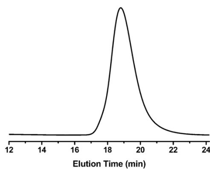
Fig. S2 Gel permeation chromatography curves of P(NBMA-co-MEO 2 MA-co-OEGMA).
