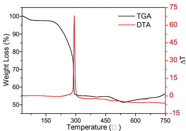
Fig. S1 TGA and DTA curves of the PZT green fiber mats
