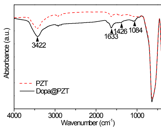
Fig. S2 FT-IR spectra of the PZT nanofibers before (dashed line) and after (solid line) dopamine modification processing.
