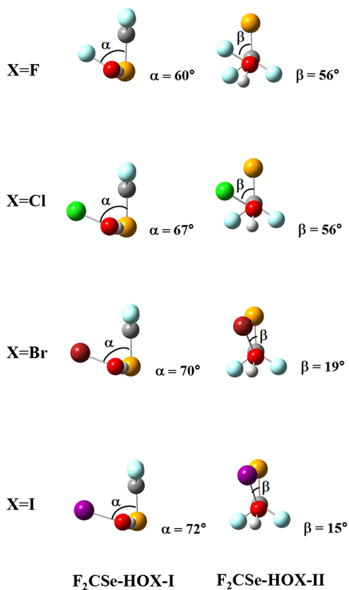
Fig. S1. Optimized structures of the complexes F 2 CSe-HOX-I and F 2 CSe-HOX-II.
