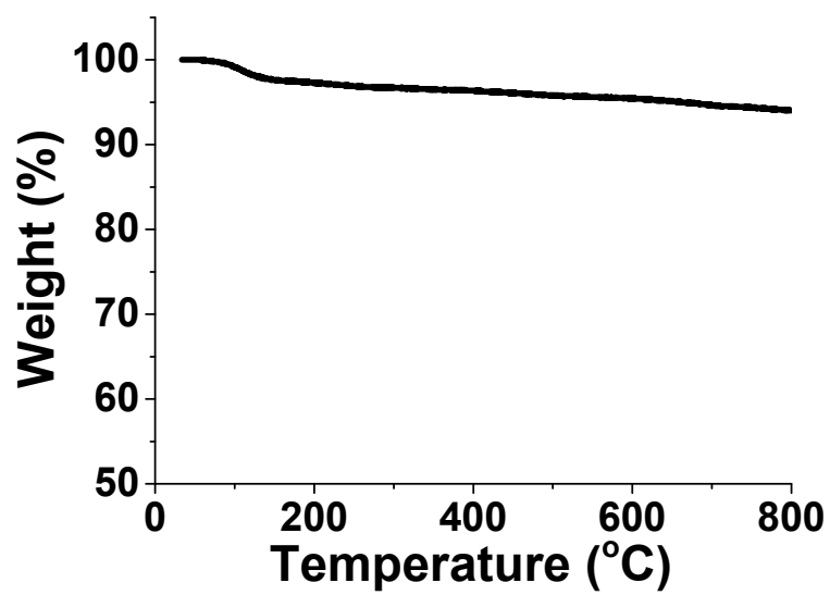
Fig. S1. TG curve of pristine vermiculite.
