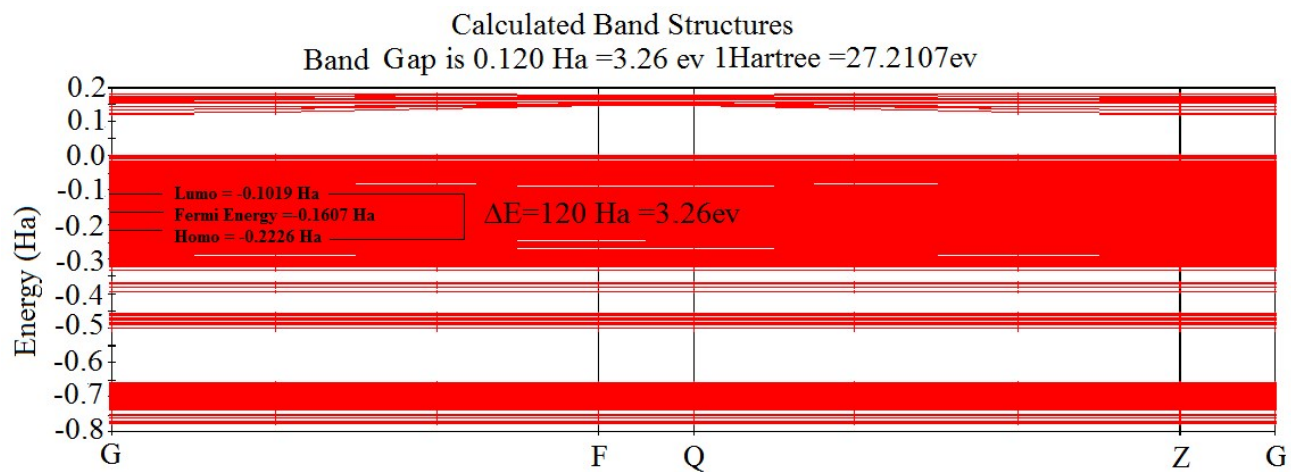
Fig S2. Plot of calculated band structure
